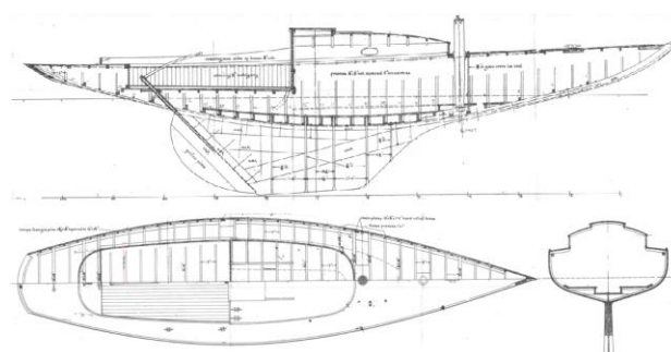
Figure 2: Structures of the Dark Harbor 17.5 [1].
