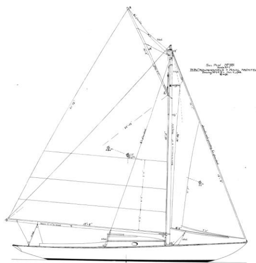
Figure 1: Sail plan of the Dark Harbor 17.5 [1].
