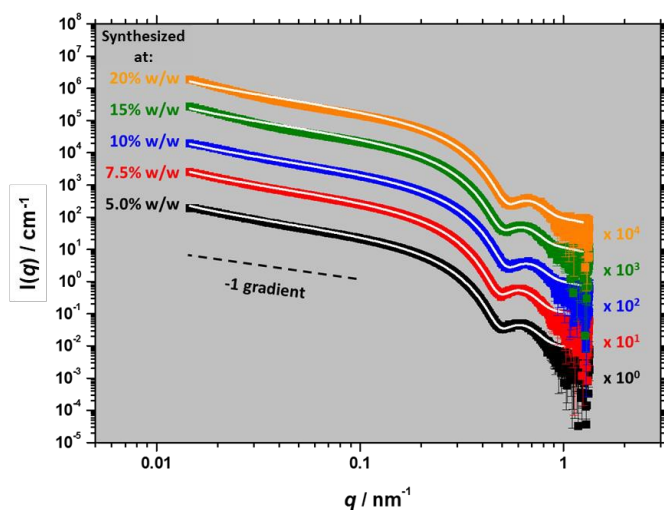
Figure 2. Representative SAXS patterns recorded at 20 °C for 1.0% w/w dispersions of PSMA 13 -PBzMA x worms prepared in mineral oil at 5.0% w/w (black symbols), 7.5% w/w (red symbols), 10% w/w (blue symbols), 15% w/w (green symbols) or 20% w/w (orange symbols). The white lines for each SAXS pattern indicate the data fit obtained when using an established worm-like micelle model (equations S1-S8). 48 Each pattern and its corresponding data fit is offset by the stated arbitrary factor for the sake of clarity.
