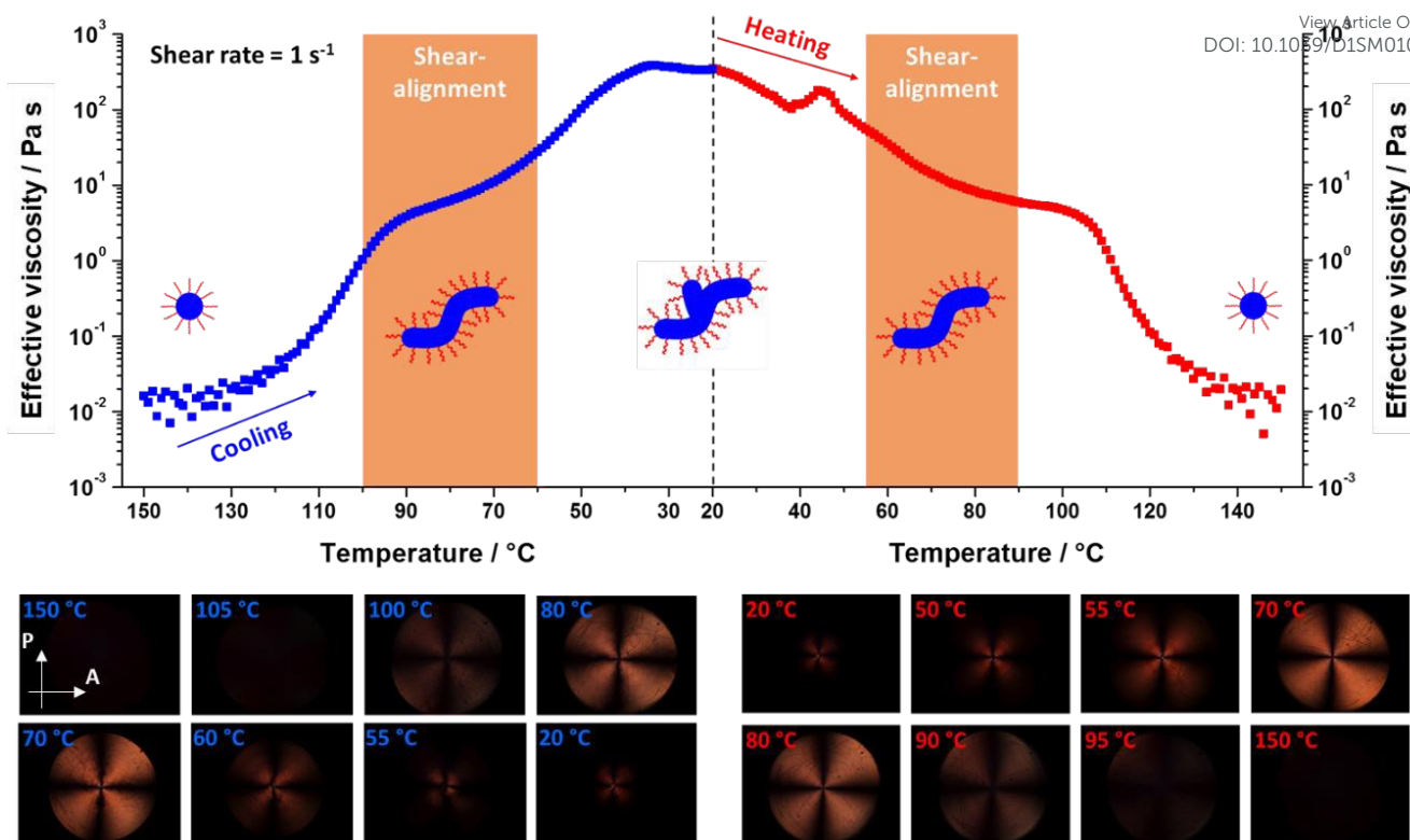
Figure 5. Dispersion viscosity-temperature profile and corresponding polarized light images (PLIs) obtained for a 20% w/w dispersion of PSMA 13 -PBzMA 64 nano-objects on cooling from 150 °C to 20 °C (blue data, left of the dashed vertical line) and on heating from 20 °C to 150 °C (red data, right of the dashed vertical line) at a rate of 2 °C min -1 when employing a constant maximum (sample edge) shear rate of 1 s -1 . Selected PLIs represent the sample birefringence observed at various temperatures (see Figure S4 for additional PLIs). Arrows show the planes of polarization for the polarizer (P) and the analyzer (A), crossed at 90°. A Maltese cross motif indicates shear-induced alignment of anisotropic objects, whereas its absence indicates either no alignment or no anisotropic objects. All PLIs recorded during the cooling cycle are shown in Figure S1. The diameter of the sample is 25 mm.
