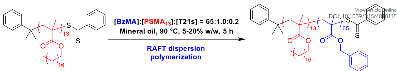
Scheme 1. Synthesis of targeted poly(stearyl methacrylate) 13 -poly(benzyl methacrylate) 65 (PSMA 13 -PBzMA 65 ) worms via RAFT dispersion polymerization of BzMA in mineral oil at 90 °C. Final copolymer concentrations ranged from 5.0 to 20% w/w solids.
