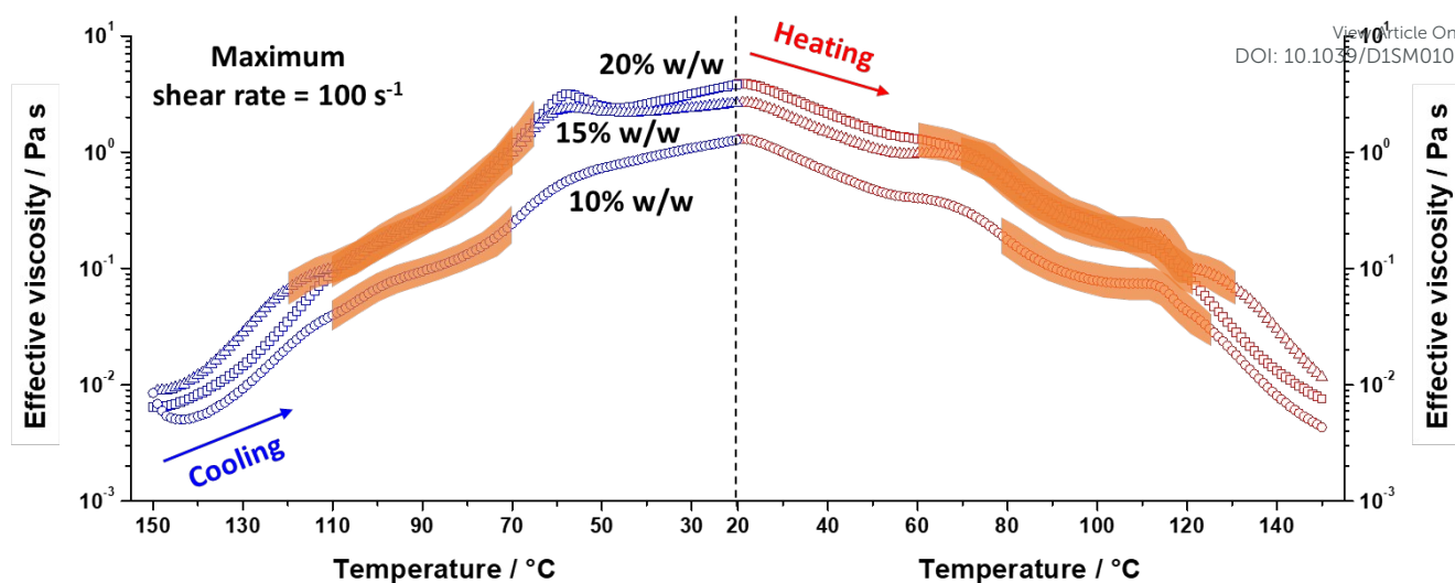
Figure 7. Combination of the dispersion viscosity-temperature profile recorded for the cooling (blue data) and heating (red data) temperature ramps (cooling/heating rate = 2 °C min -1 ) for a 20% w/w (squares), 15% w/w (triangles) and 10% w/w (circles) dispersion of PSMA 13 -PBzMA x nano-objects at the maximum (sample edge) shear rate = 100 s -1 . The highlighted regions represent the temperature ranges over which sample birefringence is observed.
