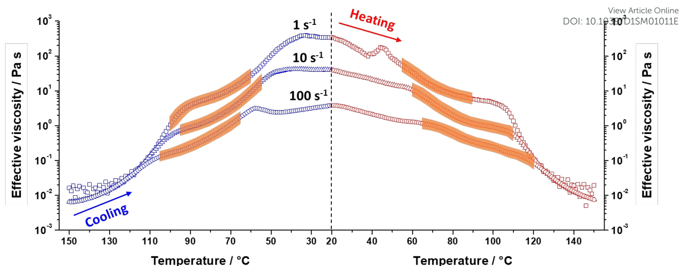
Figure 6. Combination of the dispersion viscosity-temperature profiles recorded for the cooling (blue data, left of dashed vertical line) and heating (red data, right of dashed vertical line) temperature ramps (cooling/heating rate = 2\text{ }^{\circ}\text{C min}^{-1} ) for a 20% w/w dispersion of PSMA 13 -PBzMA 64 nano-objects at the maximum (sample edge) shear rate of 1\text{ s}^{-1} (squares), 10\text{ s}^{-1} (triangles) or 100\text{ s}^{-1} (circles). The orange-shaded regions represent the temperature ranges over which sample birefringence was observed.
