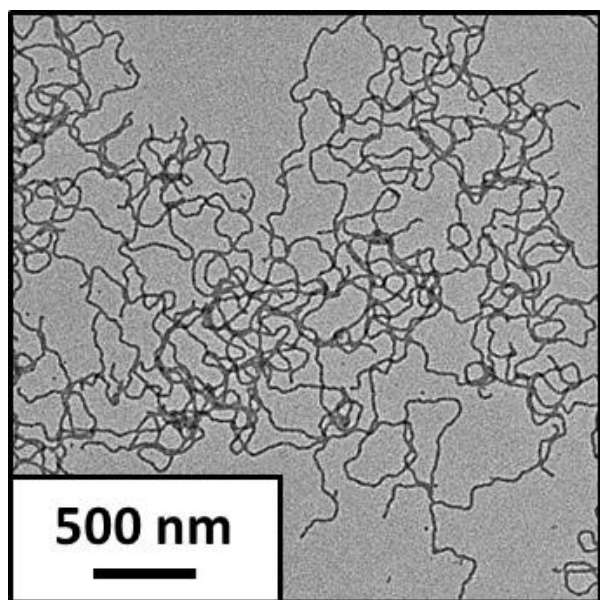
Figure 1. Representative transmission electron micrograph recorded for a 0.10% w/w dispersion of PSMA 13 -PBzMA 63 worms prepared in mineral oil at 10% w/w solids.
