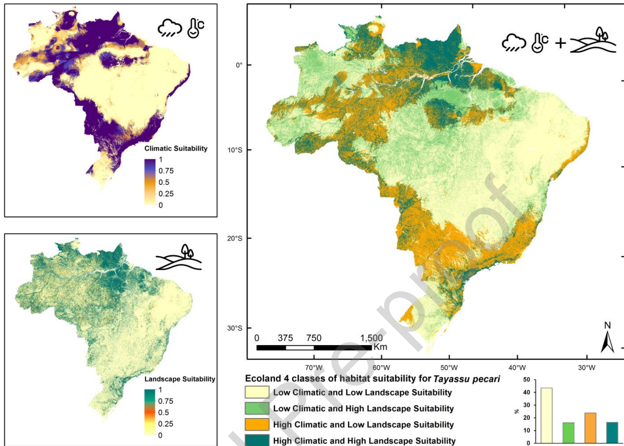
Figure 3. Climatic, Landscape, and Ecoland models of habitat suitability for white-lipped peccaries ( Tayassu pecari ) in Brazil.
