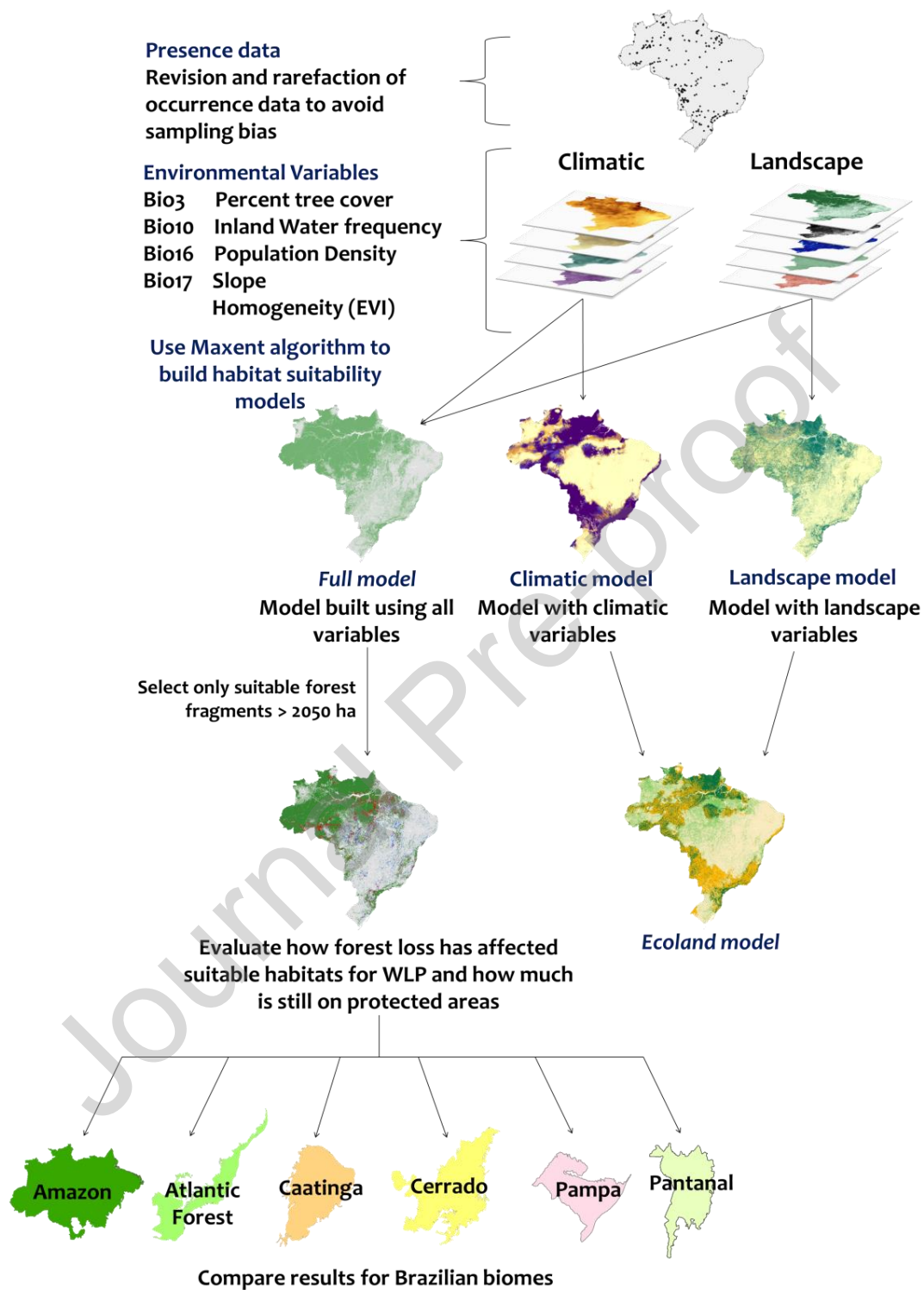
Figure 2. A conceptual framework for the Full and Ecoland models used to analyze habitat suitability for Tayassu pecari in Brazil, with the spatial analysis steps used to quantify the impact of forest loss on its distribution.
