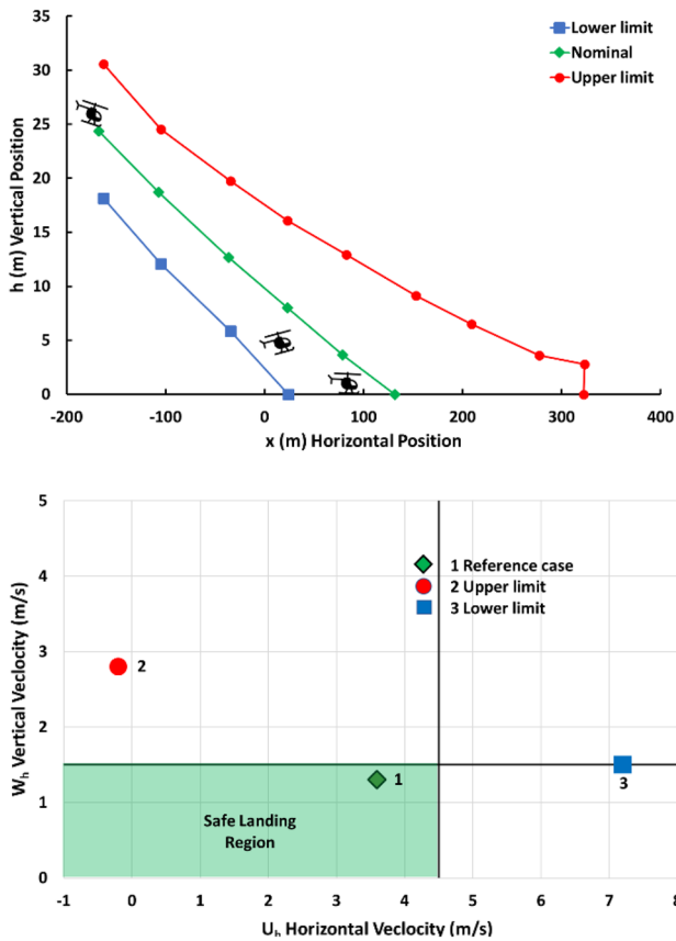
Fig. 11 Helicopter landing footprint with simulation tolerance limits [47]
