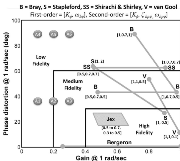
Fig. 19 Sinacori’s rotational fidelity criteria [72]
