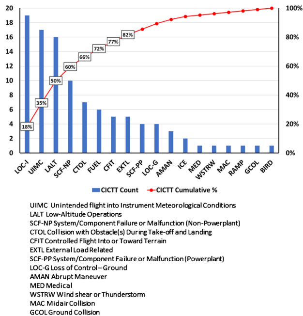
Fig. 8 Pareto chart of U.S. civil helicopter fatal accident data (2009–2013) [31]
