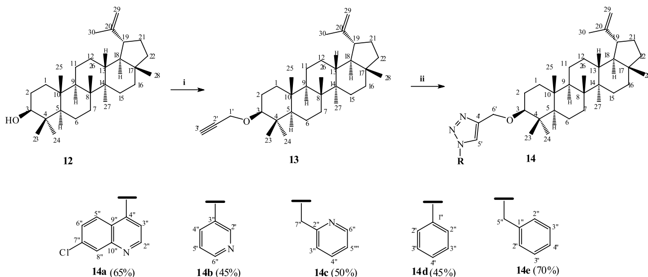
Scheme 1. Synthesis of compounds 13 and 14a-14e from lupeol ( 12 ). Reagents and conditions: (i) C_3H_5Br/NaH/THF , room temperature (r.t.), 24 h; (ii) organic azide, CuSO_4 \cdot 5H_2O (20 mol%), CH_2Cl_2/H_2O (50% v/v), r.t., 24 h. 22
