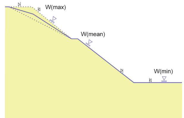
Figure 3 - Geometry of the slope and locations of minimum ( W_{min} ), maximum ( W_{max} ) and medium ( W_{mean} ) water tables.
