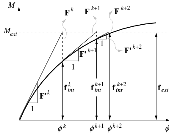
Figure 7: Moment-curvature relationship
