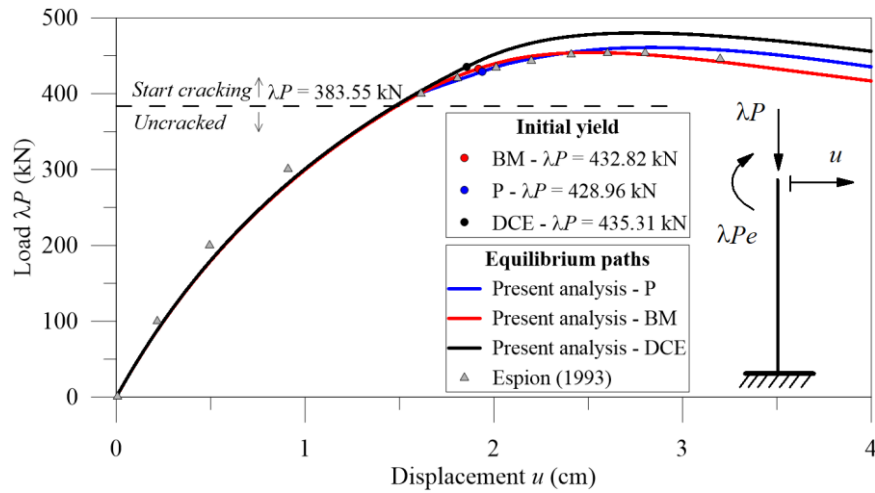
Figure 15: Foure's column: equilibrium paths comparisons using FE mesh 4
