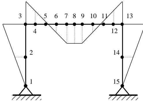
Figure 22: Bending moment diagrams: under critical load
