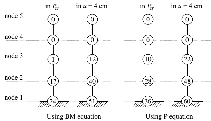
Figure 17: Percentage of the pseudo-spring rotational stiffness degradation in FE mesh 4
