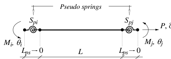
Figure 1: Hybrid finite element referenced to co-rotational system
