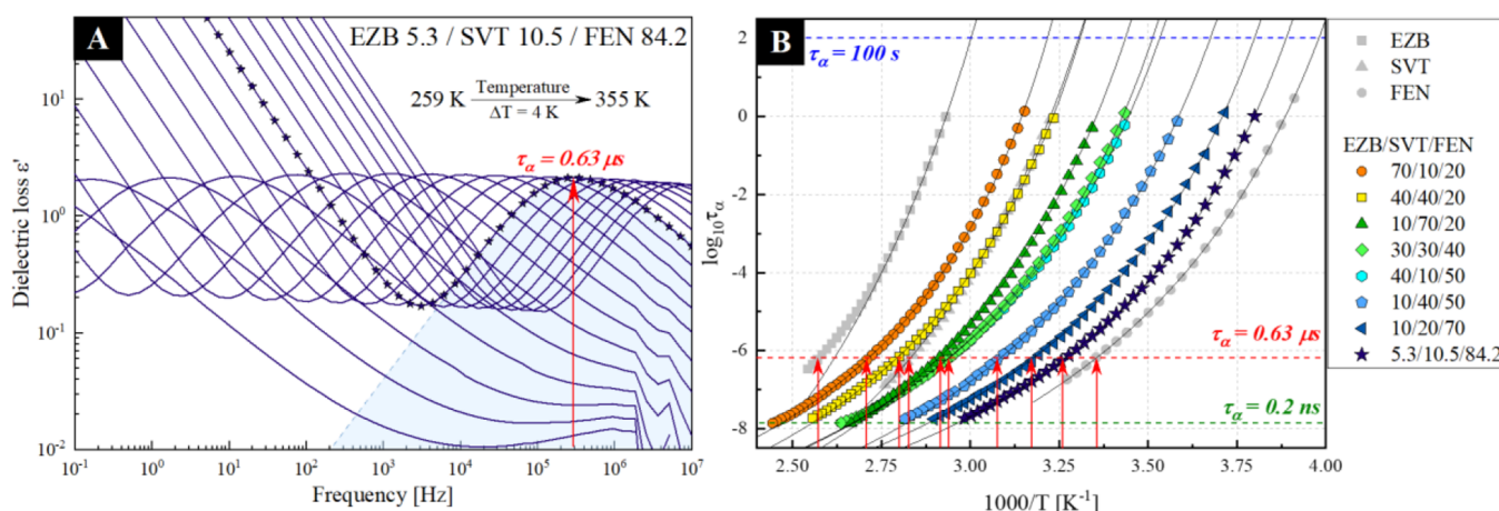
Figure 7. (a) Dielectric loss spectra collected above the glass transition temperature of ternary amorphous EZB 5.3/SVT 10.5/FEN 84.2 systems. (b) Temperature dependence of the structural relaxation times determined by using the BDS technique for pure amorphous EZB (gray squares), pure amorphous SVT (gray triangles), pure amorphous FEN (gray circles), and their ternary mixtures that contain various mass ratios of: EZB 70/SVT 10/FEN 20 (orange circles), EZB 40/SVT 40/FEN 20 (yellow squares), EZB 10/SVT 70/FEN 20 (dark green triangles), EZB 30/SVT 30/FEN 40 (light green diamonds), EZB 40/SVT 10/FEN 50 (cyan hexagons), EZB 10/SVT 40/FEN 50 (light blue pentagons), EZB 10/SVT 20/FEN 70 (dark blue triangles), and EZB 5.3/SVT 10.5/FEN 84.2 (navy stars). Solid black lines are the VFT 1 fits, dashed red line marks the region, where \tau_\alpha = 0.63 \mu\text{s} , while red arrows represent the temperatures which corresponds to \tau_\alpha = 0.63 \mu\text{s} for each sample.
