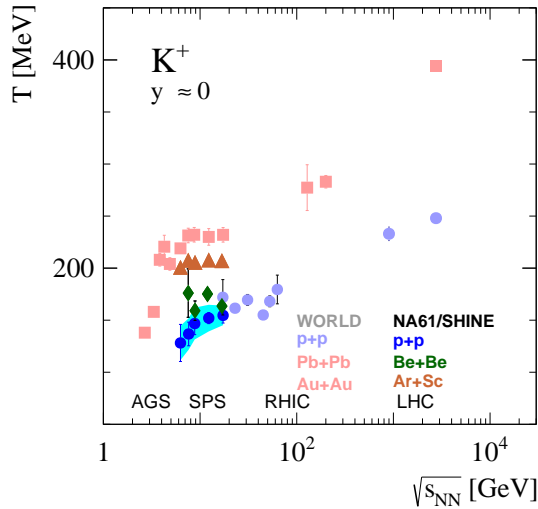
Fig. 1. Inverse slope parameter T of m_T spectra of K^+ at mid-rapidity as a function of collision energy. Most results are shown with statistical uncertainties only. For the p + p data, the shaded band indicates systematic uncertainties.
