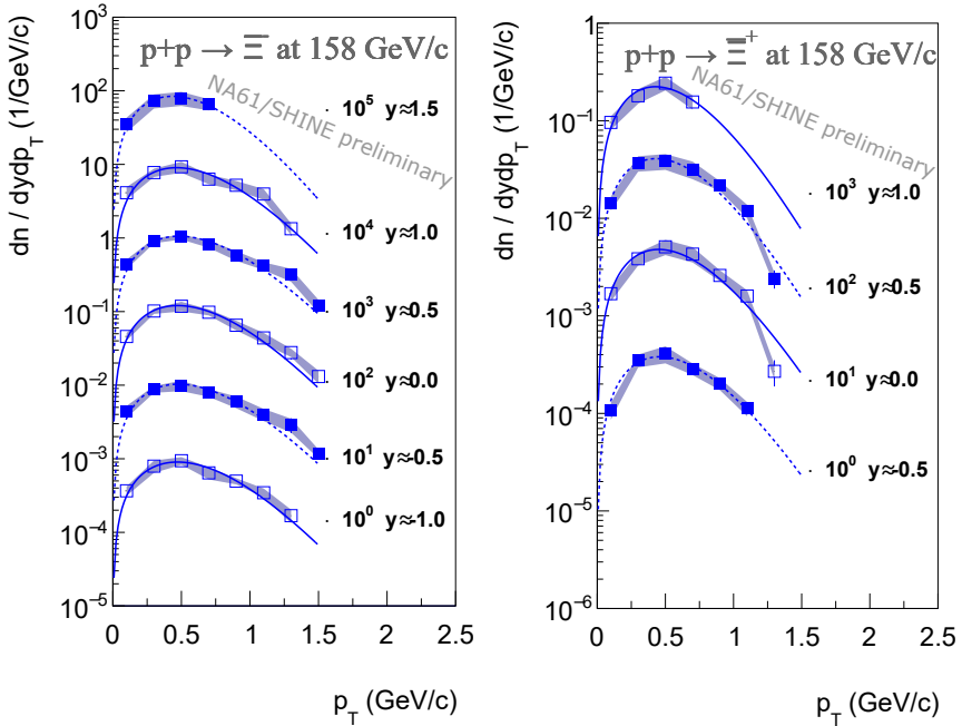
Fig. 3. (Colour on-line) Preliminary results on transverse momentum spectra of \Xi^- (left) and \Xi^+ (right) hyperons produced in inelastic p+p interactions at 158 GeV/c in consecutive rapidity bins. Results are scaled for better separation, grey bands indicate systematic uncertainty, lines (blue) exponential fits.
