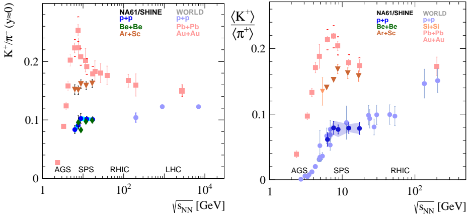
Fig. 2. Ratio of yields K^+/\pi^+ at mid-rapidity and the ratio of total yields \langle K^+ \rangle / \langle \pi^+ \rangle produced in p + p , Be+Be, Ar+Sc and Pb+Pb collisions as a function of collision energy.
