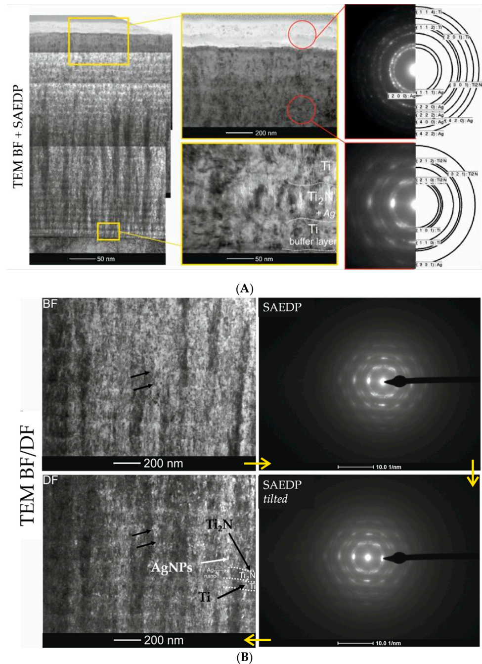
Figure 1. TEM/BF images and accompanying electron diffractions: (A) of multi-layer Ti/Ti x N coating with thickness (~3.80 μm) implanted with Ag nanoparticles (12.5% at.), (B) of Ag nanocrystallites in both Ti and Ti 2 N layers.
