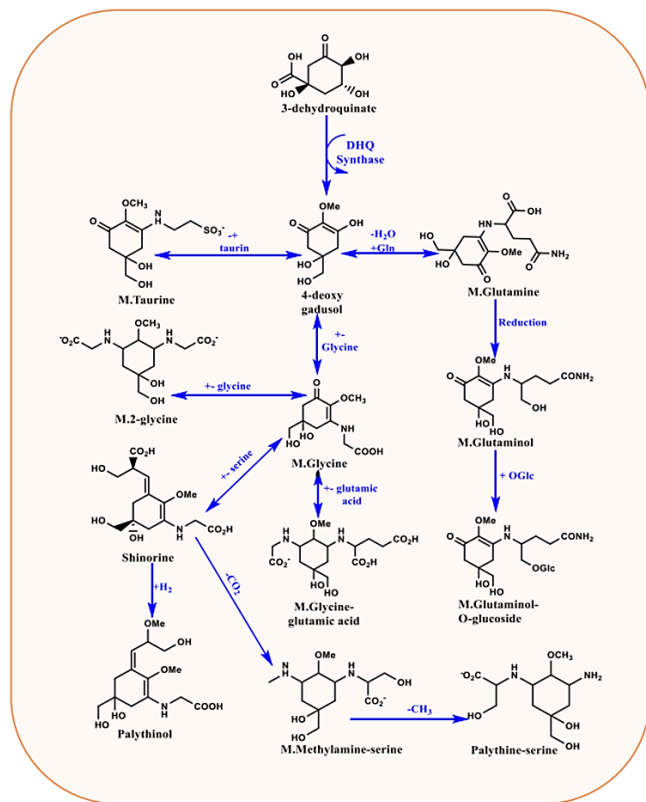
Figure 3. The 11 MAAs types synthesized from 3-dehydroquininate synthase (DHQS) and their pathway in D. radiodurans R1 bacteria. 3-dehydroquininate (DHQ) is converted to the precursor molecule, 4-deoxygadusol by the bi-functional role of DHQS. Then amino acid glycine is added to the core structure and producing primary MAAs, the M.Glycine. Different kinds of amino acid attached either to 4-deoxygadusol or M.Glycine and producing other secondary or peripheral MAAs [14].
