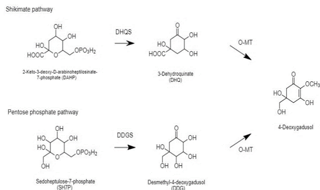
Figure 1. The possible pathway for the production of 4-deoxygadusol, the precursor for mycosporine-like amino acids (MAAs). 3-dehydroquinase synthase (DHQS) is the key enzyme in shikimate pathway which catalyses the conversion of 3-deoxy-D-arabinoheptulosonate-7-phosphate (DAHP) to 3-dehydroquininate (DHQ) while demethyl-4-deoxygadusol synthase (DDGS) is the key enzyme in pentose phosphate pathway which catalyses sedoheptulose-7-phosphate to demethyl-4-deoxygadusol (DDG). The 4-deoxygadusol will be produced upon conversion of DHQ and DDG by O-methyltransferase (OMT) .
