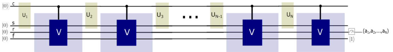
FIG. 2. Illustration of the quantum protocol. The system interacts with the different parties via a sequence of controlled entangling unitaries. Quantum control of causal order is achieved by a series of unitaries U_n on the control and system wires.
