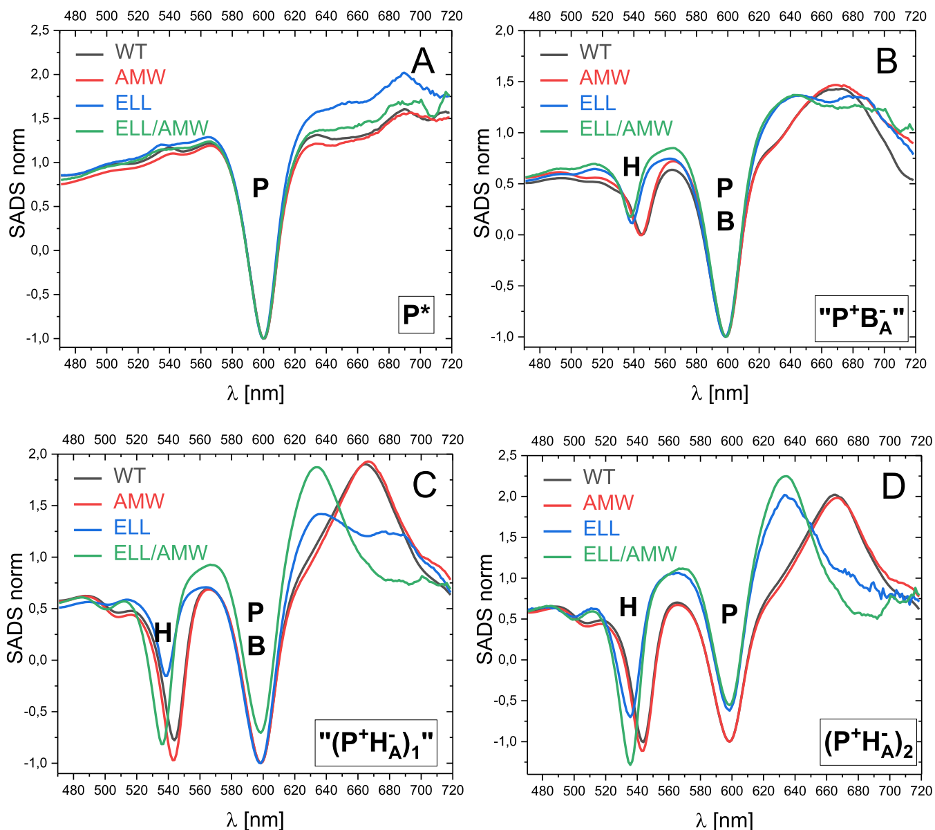
Figure 6. Comparisons of the line shapes of analogous SADS for the four RCs. (A,B) spectra of the compartments P^* and " P^+B_A^- ", respectively, normalized at \sim 600 nm and (C,D) spectra of the compartments " (P^+H_A^-)_1 " and " (P^+H_A^-)_2 " normalized in such a way that the depth of the \sim 600 nm PB band relative to the amplitude at 565 nm is the same for all the samples.
