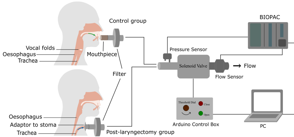
Fig. 3. System design of RoboCough.
