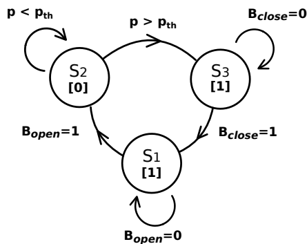
Fig. 6. System state diagram relative to user input, where states S_1, S_2 and S_3 correspond to the phases of inhale, compression and exhale (cough) shown in Fig 2, and valve states are represented by [0] for close and [1] for open. State transitions are governed by pressure threshold p_{th} and button presses.
