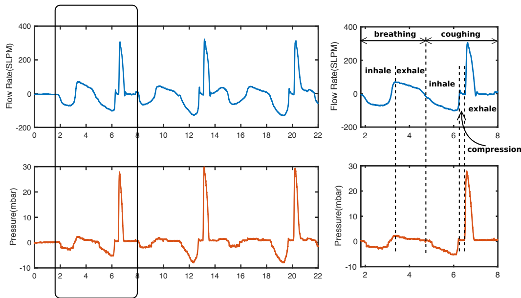
Fig. 2. Flow rate and respiratory mouth pressure during three consecutive coughs by participants with a single cough profile enlarged on the right.
