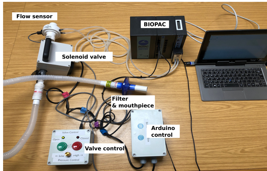
Fig. 4. Photograph of the RoboCough test and evaluation system.
