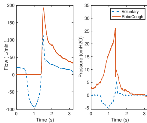
Fig. 8. Example cough flow and pressure profiles from post-laryngectomy group during voluntary and RoboCough assisted cough.
