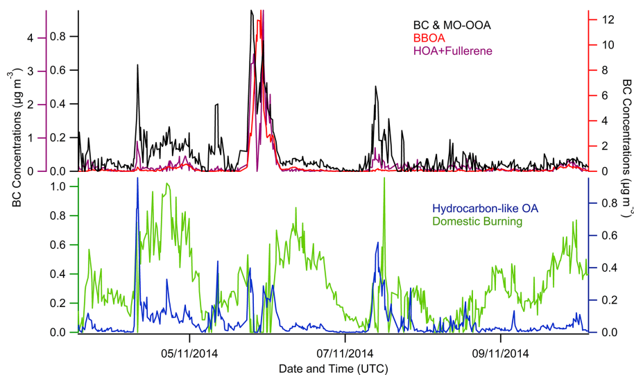
Figure 7. The contributions of BC signals in \mu\text{g}/\text{m}^3 after normalising it to the concentrations of eBC 950 from the Aethalometer (AE31) (Reyes-Villegas et al., 2018).
