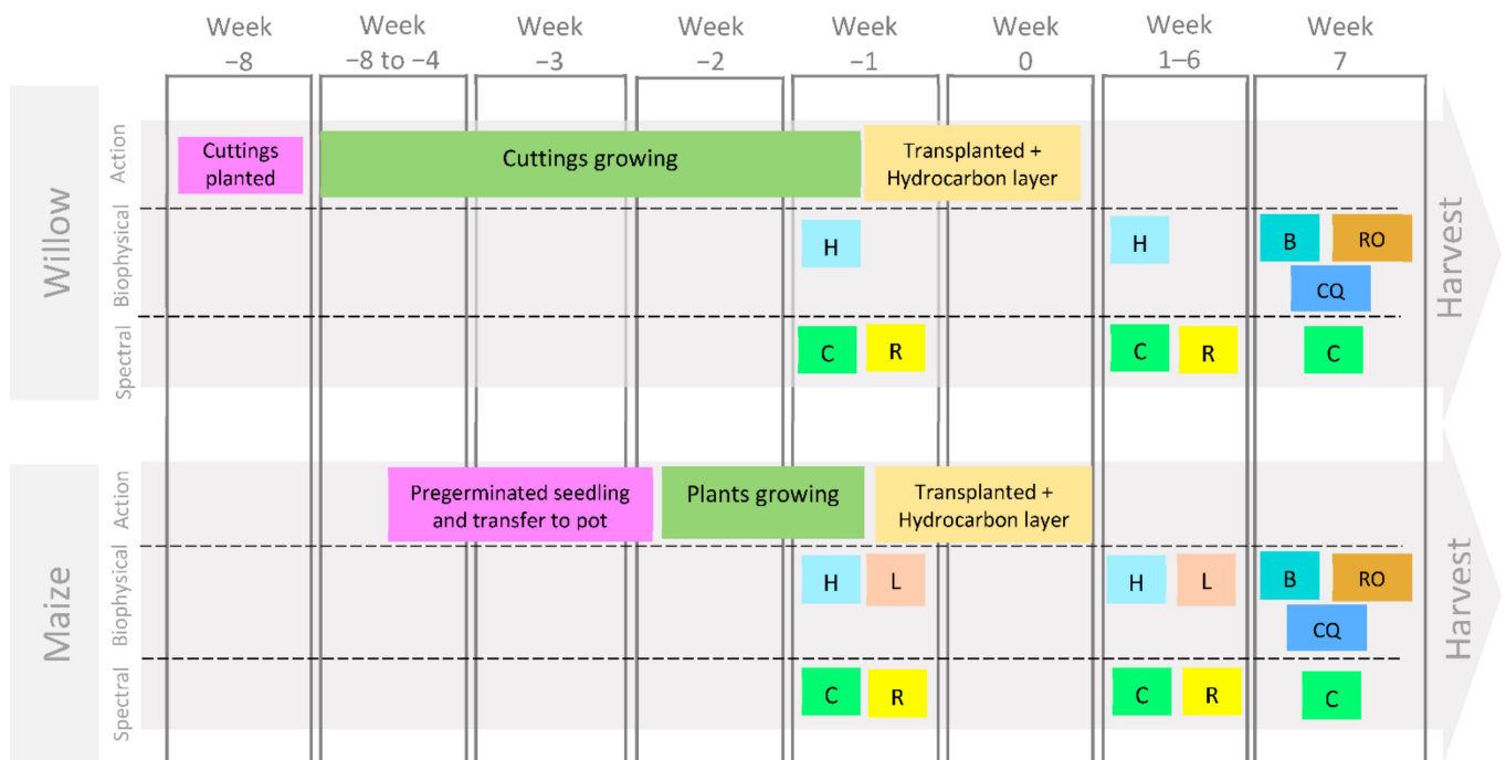
Figure 1. Experiment steps (Action), biophysical and spectral data collection for willow and maize. (L = leaf number, including colour; H = plant height, C = chlorophyll measured with MultispeQ, R = reflectance measured with ASD FieldSpec ® Pro 3, B = total plant biomass, RO = root observations, CQ = chemical analysis of chlorophyll).
