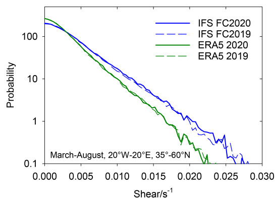
Figure 5. Probability density of vertical shear of horizontal wind normal to flight segments along the traffic routes over Europe as in 2020, evaluated separately for the FC and ERA5 meteorology as in Fig. 4.
