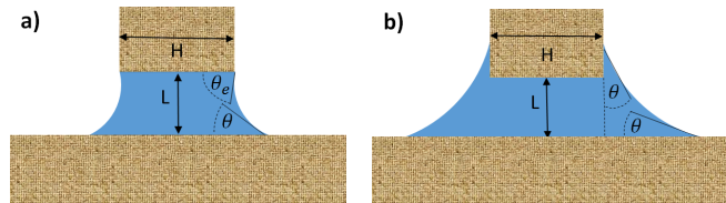
FIG. 1: Schematic illustration of two possible capillary liquid (CL) configurations in which the menisci a) are pinned at the top corners with edge contact angle \theta_e , b) spill out of the slit meeting the walls with Young’s contact angle \theta .
