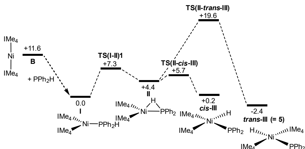
Figure 6. Computed free energy profile [kcal/mol, B97D(benzene, BS2)//BP86(BS1)] for the reaction of [Ni(IME 4 ) 2 ] ( B ) with PPh 2 H to form trans -[Ni(IME 4 ) 2 (PPh 2 )H] 5 . The triplet form of [Ni(IME 4 ) 2 (PPh 2 )H], 3 III , is computed at +23.7 kcal/mol.
