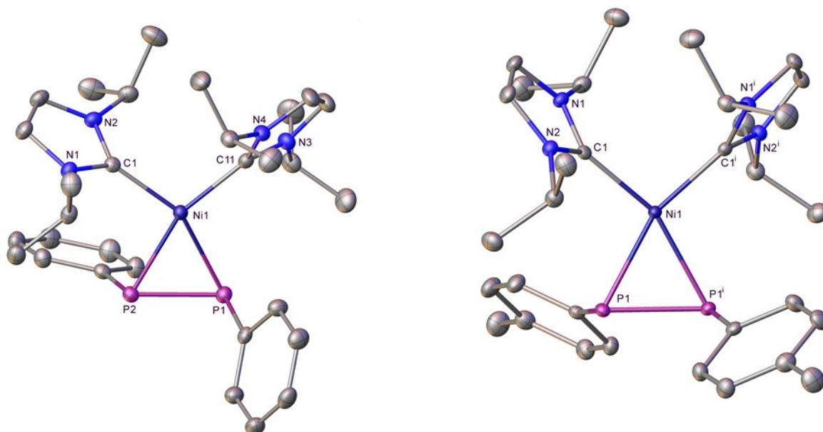
Figure 5. Molecular structures of [\text{Ni}(\text{I}'\text{Pr})_2(\eta^2\text{-PhP=PPh})] ( 18 ) and [\text{Ni}(\text{I}'\text{Pr})_2\{\eta^2\text{-(para-Tol)P=P(para-Tol)}\}] ( 19 ). Ellipsoids are represented at 30% probability and hydrogens (along with lattice solvent in 19 ) have been omitted for clarity. For 19 : i 1 - x, y, \frac{1}{2} - z symmetry operation.
