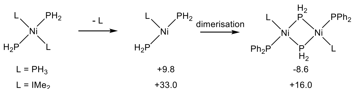
Scheme 10. Computed free energies [kcal/mol, B97D(benzene, BS2)//BP86(BS1)] for ligand loss and dimerization in trans -[NiL 2 (PH 2 ) 2 ] (L = PH 3 , IMe 2 ).
