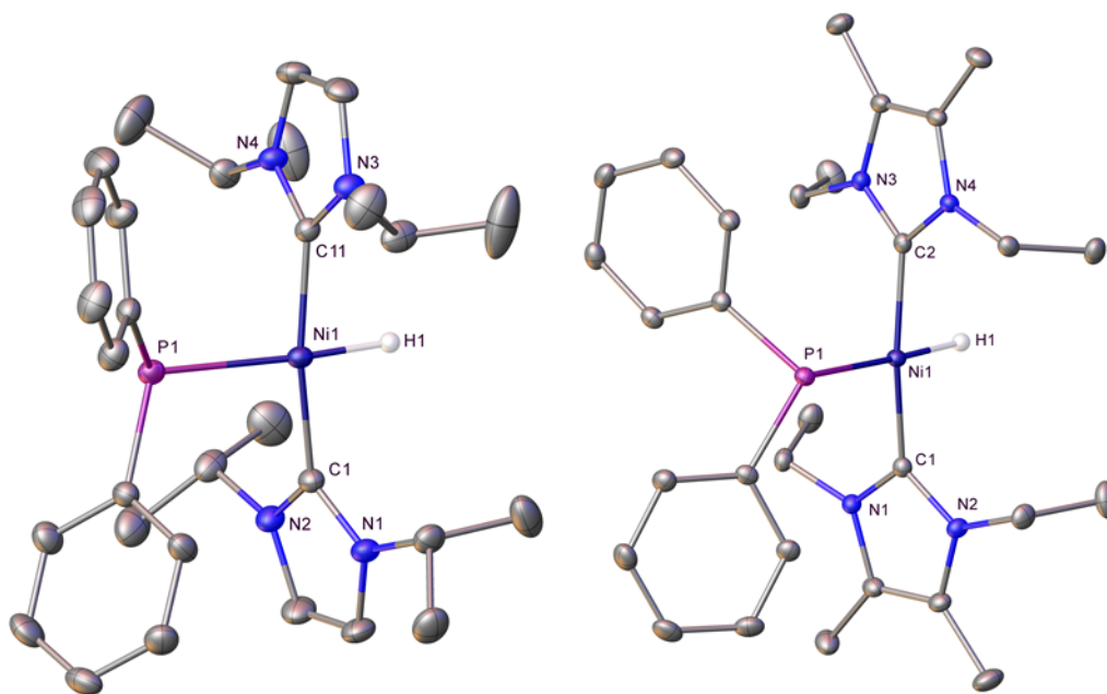
Figure 2. Molecular structures of (left) trans -[Ni(I'Pr) 2 (PPh 2 )H] ( 3 ) and (right) trans -[Ni(IEt 2 Me 2 ) 2 (PPh 2 )H] ( 4 ). Ellipsoids are shown at 30% probability with all hydrogen atoms, except Ni-H, removed for clarity.
