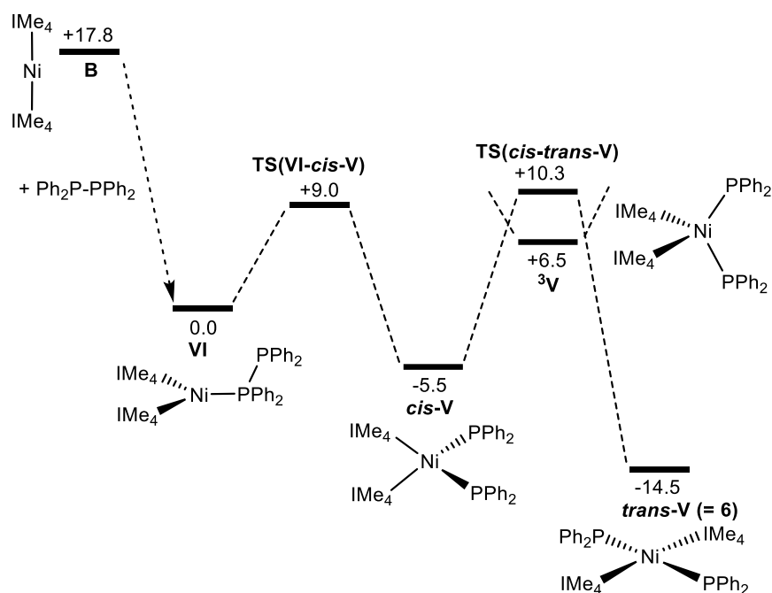
Figure 10. Computed free energy profiles [kcal/mol, B97D(benzene, BS2)/BP86(BS1)] for the reaction of B with \text{Ph}_2\text{P-PPh}_2 to form 6 .
