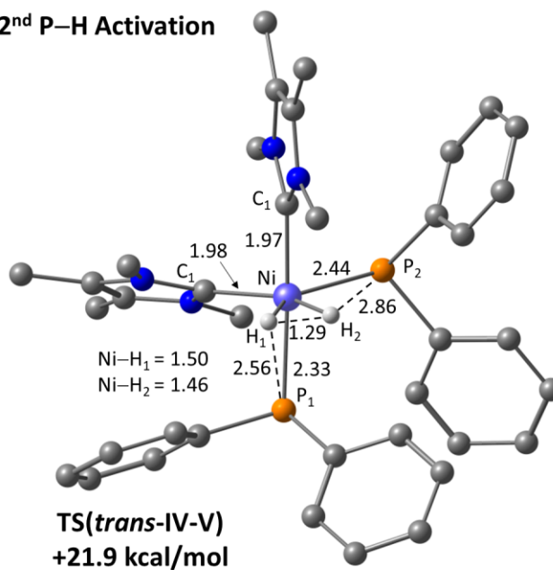
Figure 7. Computed geometries for the rate-limiting transition states for the first and second P-H activation of \text{PPh}_2\text{H} at B . Selected distances are shown in Å, with \text{IMe}_4 and phenyl hydrogens omitted for clarity.
