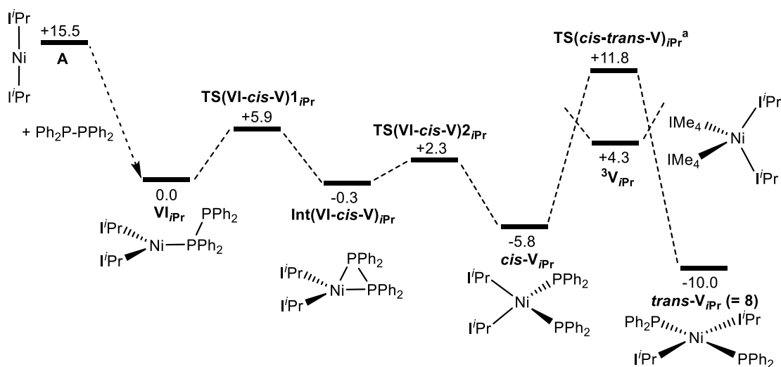
Figure 12. Computed free energy reaction profile [kcal/mol, B97D(benzene, BS2)//BP86(BS1)] for the reaction of A with Ph 2 P-PPh 2 to form trans -[Ni( i Pr) 2 (PPh 2 ) 2 ], 8 ; a only the rate-limiting transition state for cis-trans isomerisation is indicated (see Figure S78 in the Supporting Information for more details).
