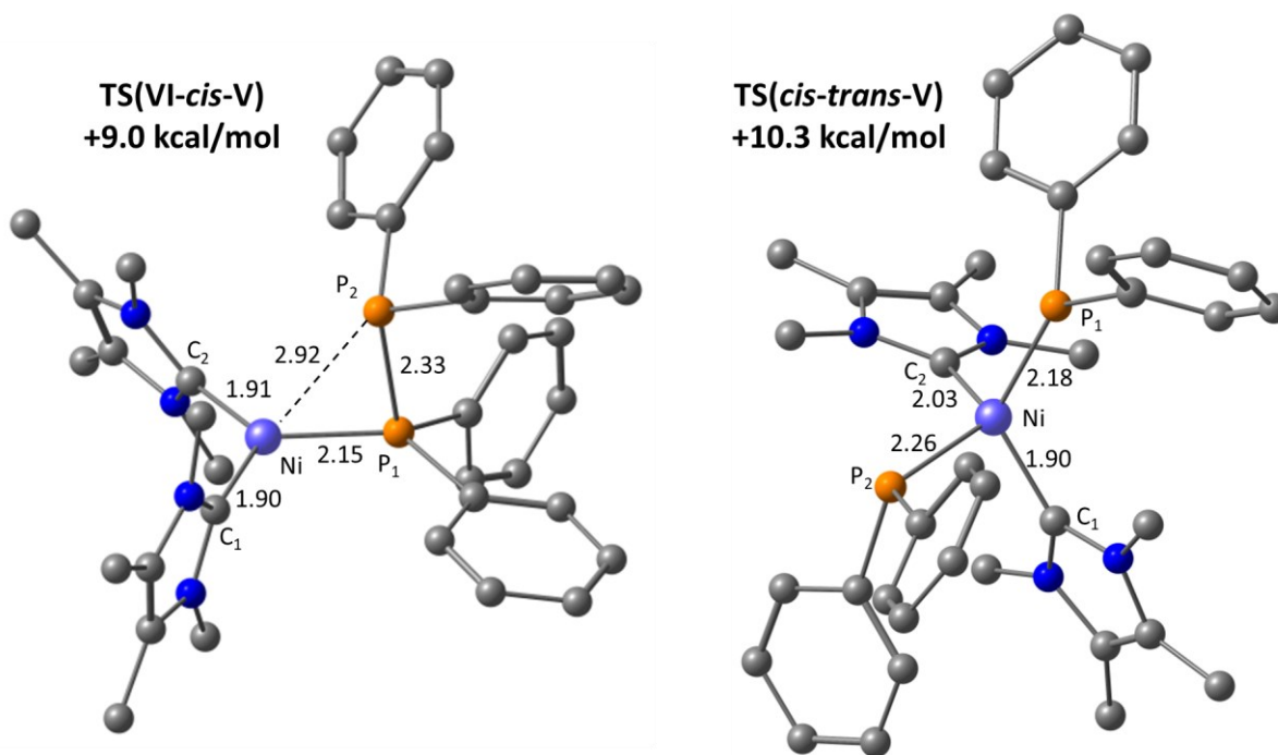
Figure 11. Computed geometries for key transition states in the P-P bond activation of \text{Ph}_2\text{PPPPh}_2 at B . Selected distances are shown in Å, with \text{IMe}_4 and phenyl hydrogens omitted for clarity.
