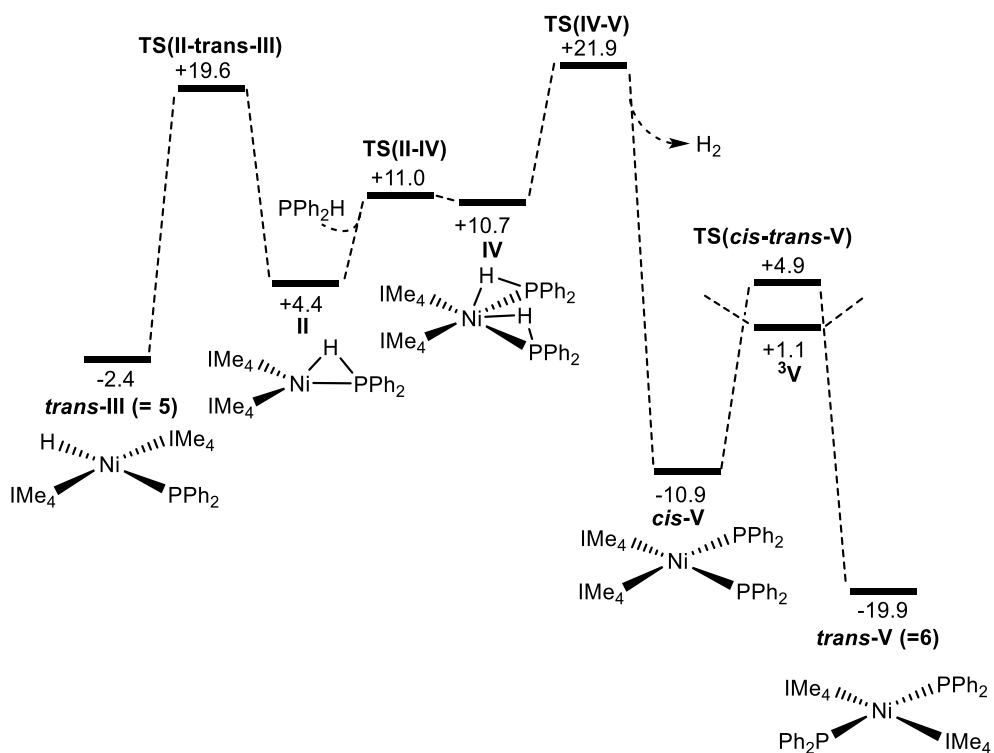
Figure 8. Computed free energy profile [kcal/mol, B97D(benzene, BS2)//BP86(BS1)] for the reaction of 5 with \text{PPh}_2\text{H} to form trans - [\text{Ni}(\text{IMe}_4)_2(\text{PPh}_2)_2] 6 .
