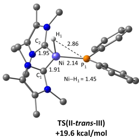
Figure 7. Computed geometries for the rate-limiting transition states for the first and second P-H activation of \text{PPh}_2\text{H} at B . Selected distances are shown in Å, with \text{IMe}_4 and phenyl hydrogens omitted for clarity.
