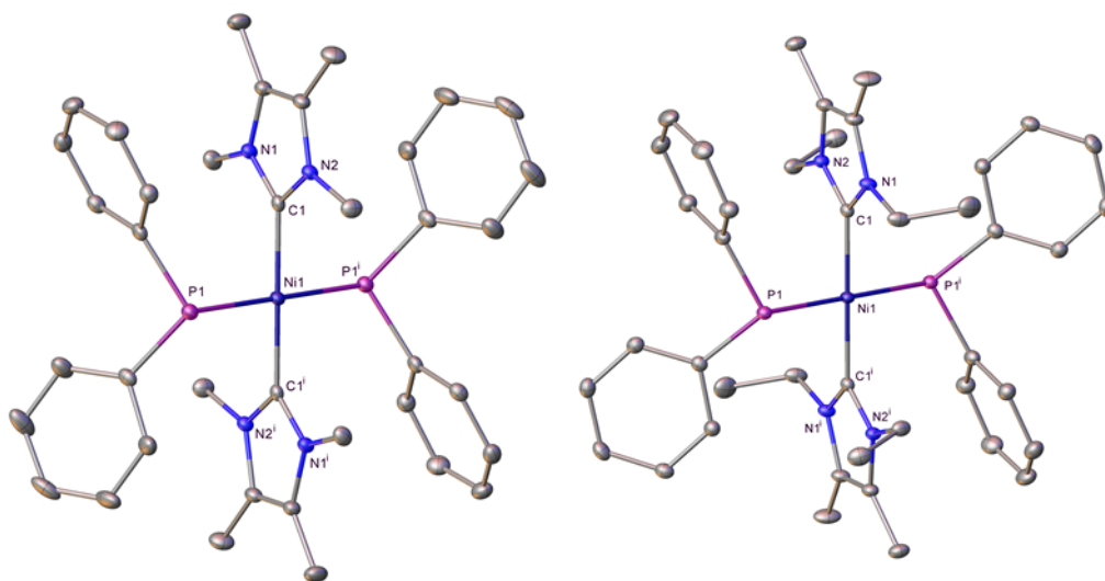
Figure 3. Molecular structures of trans -[Ni(IME 4 ) 2 (PPh 2 ) 2 ] ( 6 ) and trans -[Ni(IET 2 Me 2 )(PPh 2 ) 2 ] ( 7 ). Ellipsoids are shown at 30% probability and all hydrogen atoms are removed for clarity ( 6 ; i symmetry operation 1 - x, - y, 1 - z symmetry operation: 7 ; i symmetry operation 1 - x, 1 - y, 1 - z).
