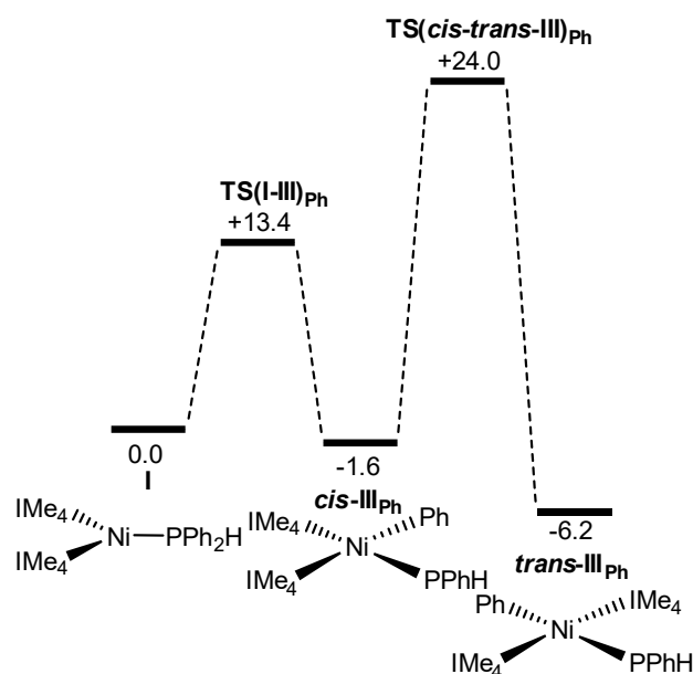
Figure 9. Computed free energy profile [kcal/mol, B97D(benzene, BS2)//BP86(BS1)] for competing P-C bond activation in [\text{Ni}(\text{IME}_4)_2(\text{PPh}_2\text{H})] , I . The triplet form of [\text{Ni}(\text{IME}_4)_2(\text{PPh}_2\text{Ph})] , ^3\text{IV}_{\text{Ph}} , is computed at +25.6 kcal/mol.
