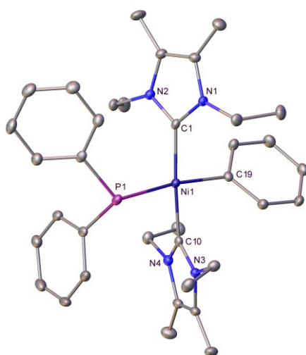
Figure 1. Molecular structure of trans - [\text{Ni}(\text{IEt}_2\text{Me}_2)(\text{PPh}_2)\text{Ph}] ( 2 ). Ellipsoids are shown at 30% probability with all hydrogen atoms removed for clarity.
