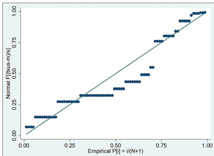
Figure 1: Outliers
