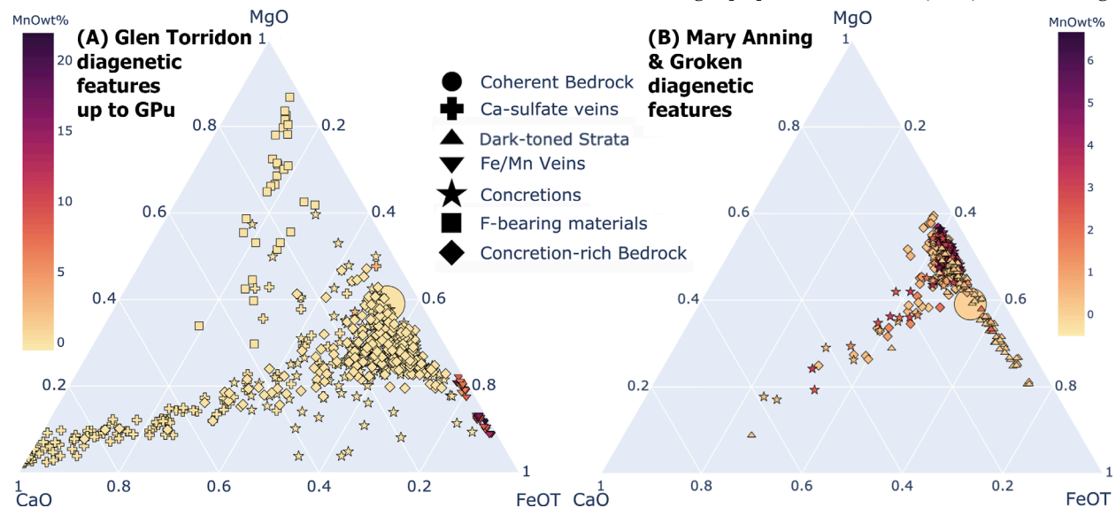
Fig 2: A) Major element oxide chemistry (moles) of the diagenetic features for the traverse from sol 2300 to the base of GPU, where colors represent wt.% MnO. B) Major element chemistry of the diagenetic features at the Mary Anning and Groken drill location.
