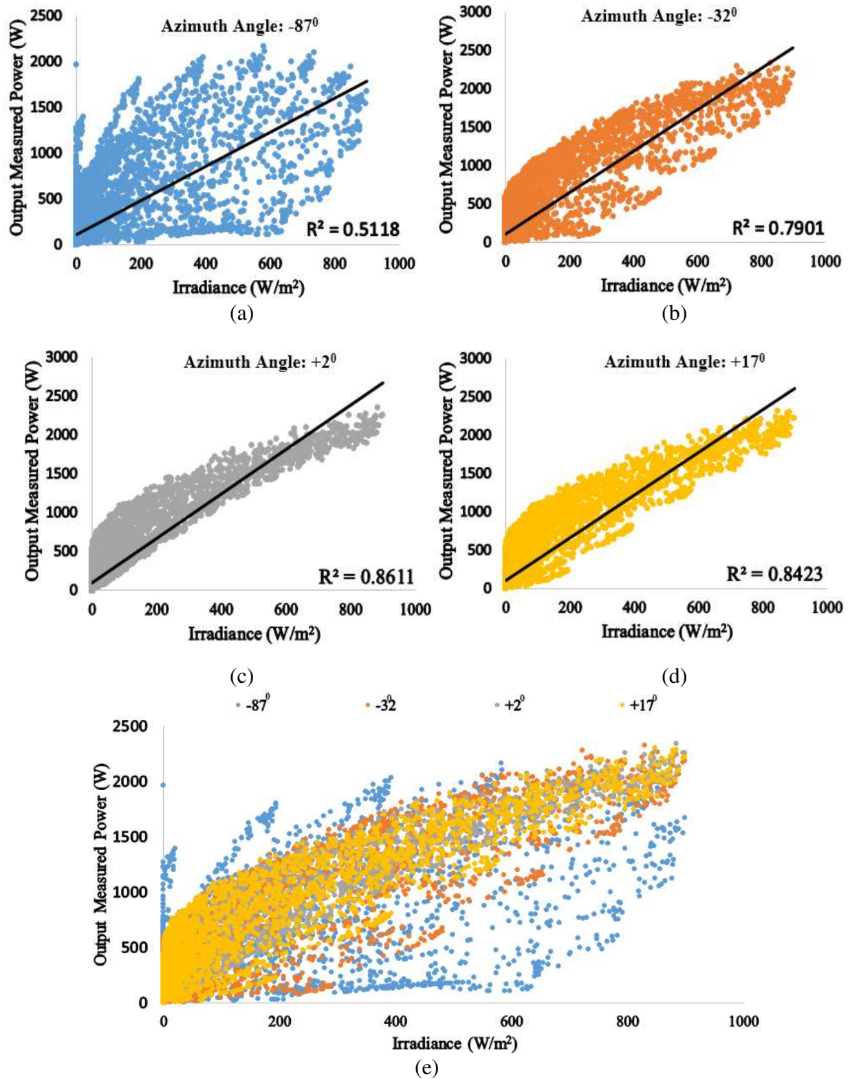
Fig. 6 Irradiance vs. output measured power obtained in PV site B. (a) PV system azimuth angle: -87^{\circ} , (b) PV system azimuth angle: -32^{\circ} , (c) PV system azimuth angle: +2^{\circ} , (d) PV system azimuth angle: +17^{\circ} , (e) Overlapping between all PV site B data
