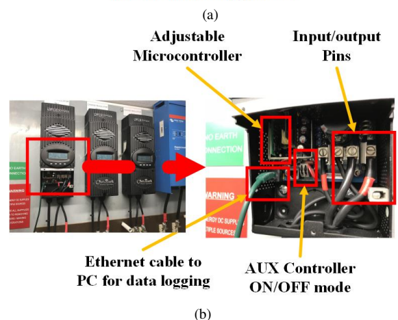
Fig. 9. (a) Examined PV system real and thermal image, (b) Internal configuration of the MPPT unit
