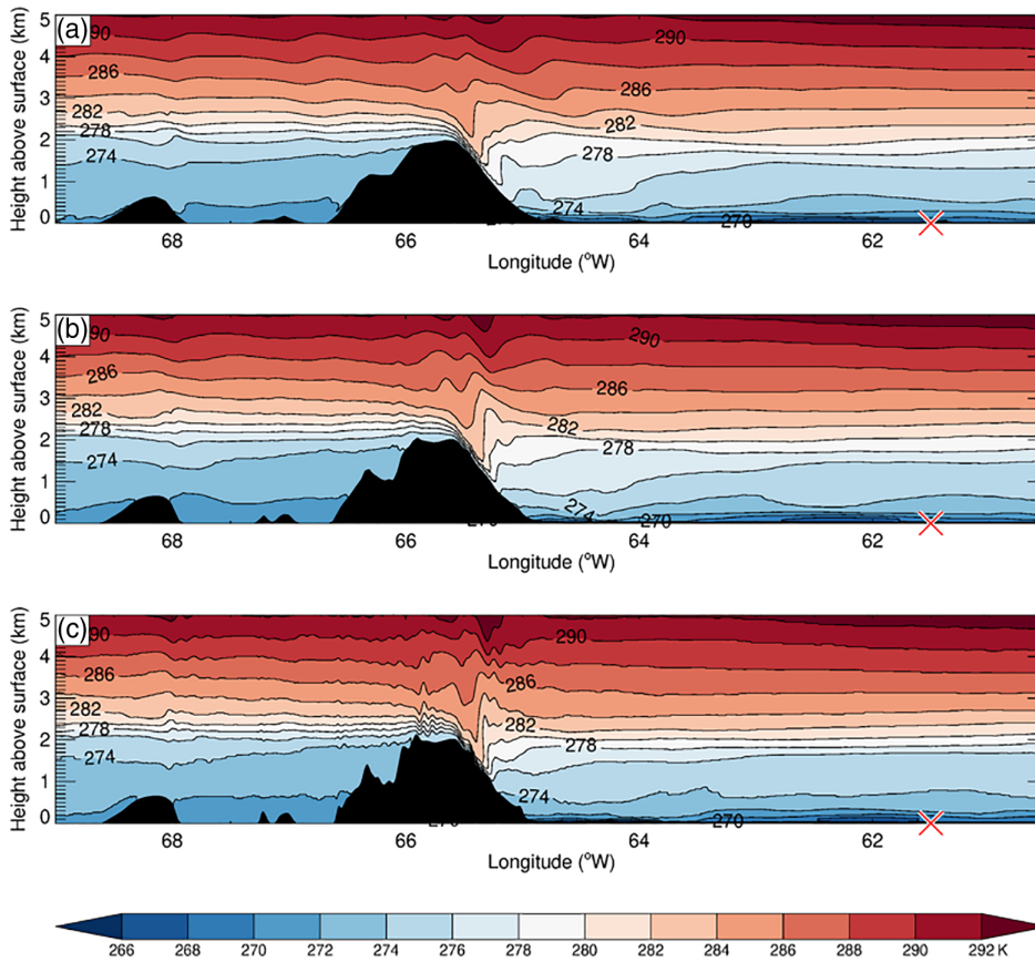
FIGURE 7 Vertical cross-sections of the MetUM simulated hourly-averaged potential temperature (K, contours) along transect “B” in Figure 1 during the foehn wind case-study at 1200 UTC (0900 LT) on 27 January 2011 at horizontal resolutions of (a) 4 km, (b) 1.5 km and (c) 0.5 km. The cross-section runs from west to east (from 69° to 60.5°W) at latitude 67.01°S and cuts through the location of AWS1, which is marked by the red cross in the panels (and located at 67.01°S, 61.5°W). The case-study is associated with west-to-east flow across the Antarctic Peninsula, so in the panels the wind is blowing from left to right. The MetUM results are based on hourly averaged output saved at T + 12 hr from a run initialised at 0000 UTC on 27 January 2011 [Colour figure can be viewed at wileyonlinelibrary.com]
