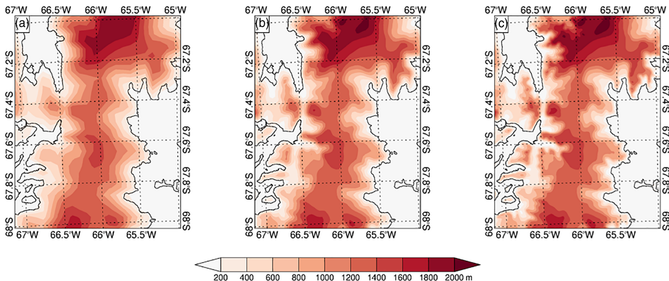
FIGURE 8 Comparison of the MetUM orography at (a) 4 km, (b) 1.5 km and (c) 0.5 km, for the Whirlwind Inlet region (labelled WI in Figure 1) [Colour figure can be viewed at wileyonlinelibrary.com ]
