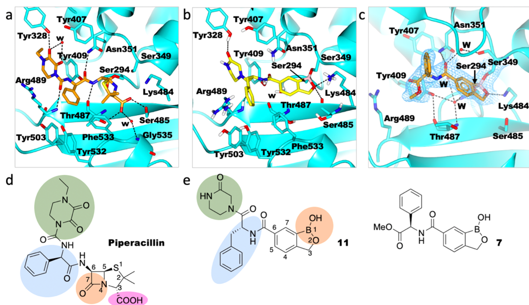
Figure 4. Binding mode of PaBPB3 inhibited by piperacillin compared with those for benzoxaboroles 7 and 11 . (a) PaBPB3 inhibited by piperacillin (PDB: 6R3X); 51 (b) predicted binding mode of 11 as determined by docking, showing how groups 1 and 2 may engage in the same manner as analogous groups in piperacillin; (c) binding mode of 7 complexed with PaBPB3 (PDB: 7AU0). Hydrogen bonds are shown as black dashed lines. An unbiased omit Fo-Fc map is shown (light blue mesh) of the ligand and covalently attached residue side chains (contoured at 1\sigma ), as calculated by “comit” in the ccp4 suite. 45 (d) Structure of piperacillin colored according to its functional groups: \beta -lactam (orange), C-3 carboxylate (pink), group 1 (blue), and group 2 (green); (e) benzoxaborole 11 was designed to mimic the piperacillin binding mode. Colors match analogous groups within piperacillin which were hoped would engage the same parts of the protein in the case of 11 .
