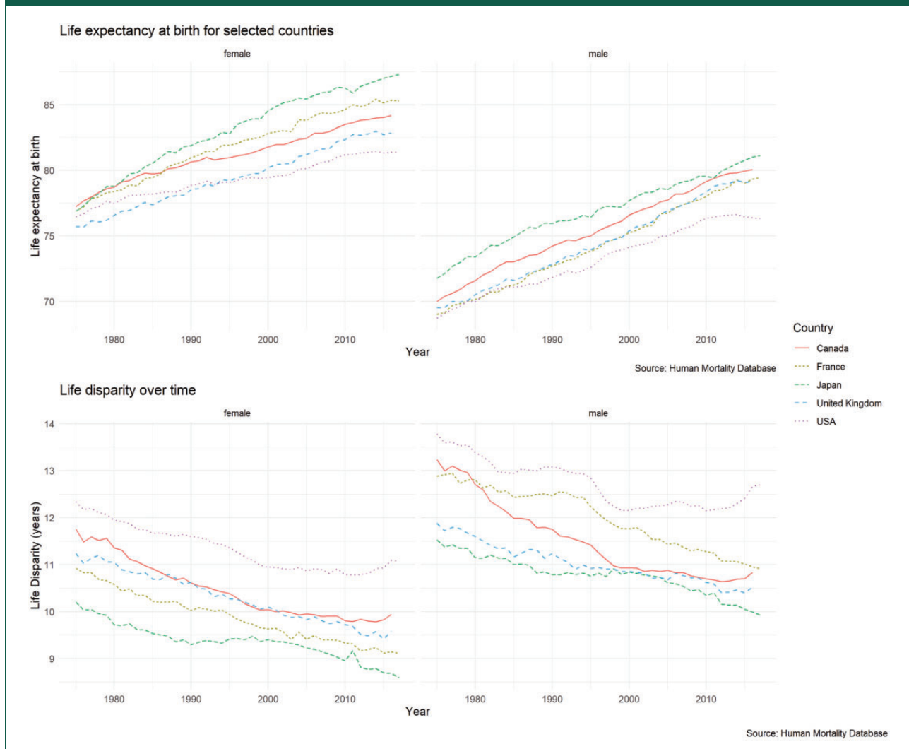
Figure 2. Life expectancy at birth (top) and life disparity over time (bottom), 1975–2017.
