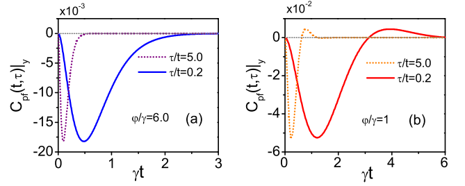
FIG. 2: (Dimensionless) CPF correlation [Eq. (36)] corresponding to the eternal non-Markovian trigonometric model [Eq. (23)], for different values of \varphi/\gamma and measurement time-interval relations \tau/t . In all cases, the system initial condition is such that \langle x \rangle = 0 .
