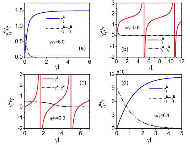
FIG. 1: Renormalized time-dependent rates [Eqs. (25) and (26)] corresponding to the multipartite trigonometric eternal non-Markovian evolution [Eq. (23)] for different values of the rate ratio \varphi/\gamma .
