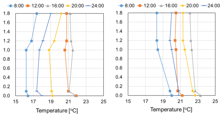
Fig. 10. Vertical temperature distributions at point B (Perimeter zone, left) and point C (Interior zone, right) indicated in Fig. 5 on February 8 th in 2019.
