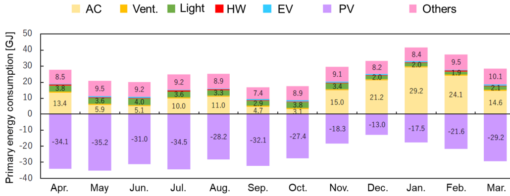
Fig. 7. Monthly primary energy consumption in FY2018
