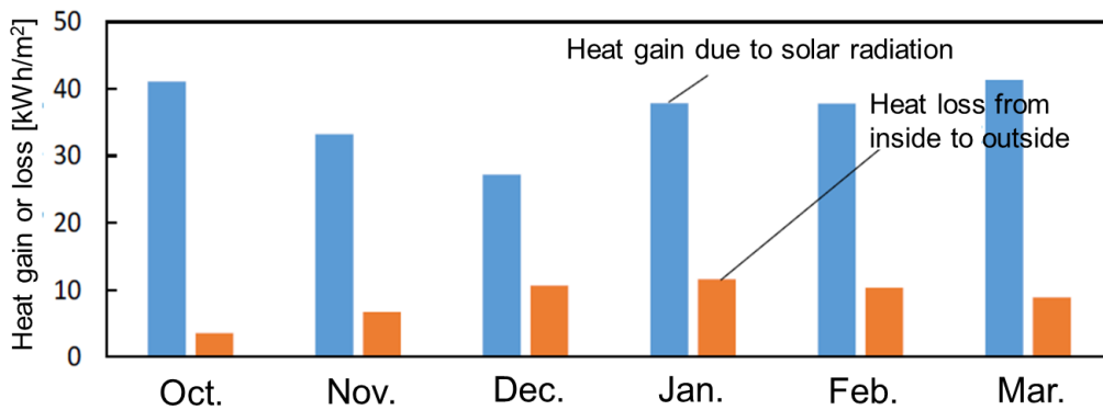
Fig. 14. Amount of heat gain due to solar radiation and heat loss due to transmission
