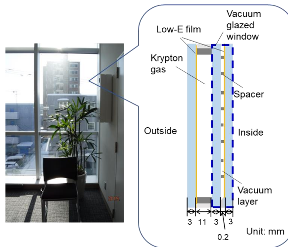
Fig. 4. Outlines of vacuum glazed window
