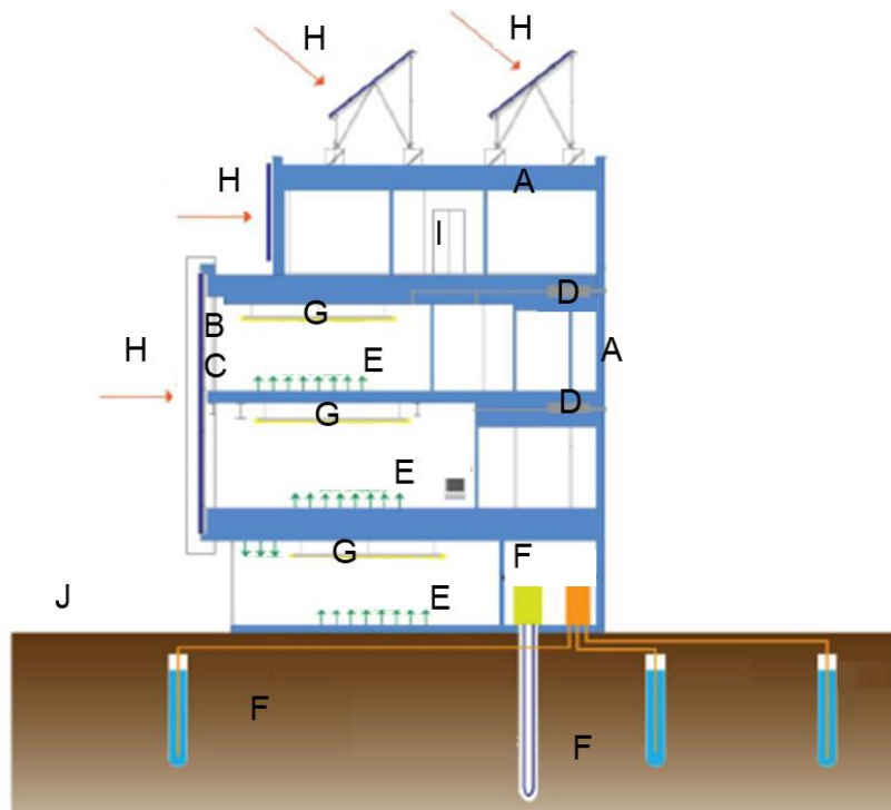
Fig. 2. Energy saving technologies installed in the office building
