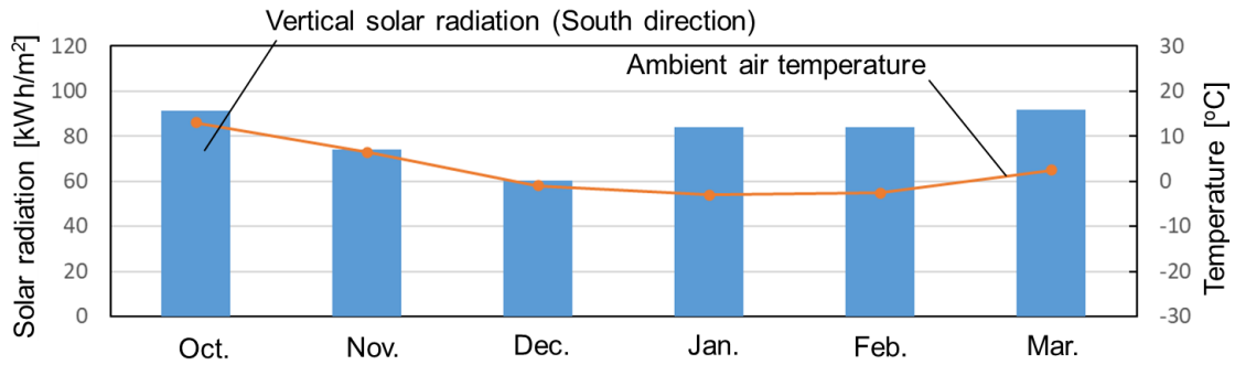
Fig. 13. Monthly average ambient air temperature and vertical solar radiation on the south side
