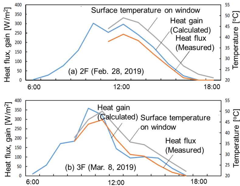
Fig. 12. Variations of variations of heat flux, surface temperature on window, and calculated heat gain ((a) 2F (Feb. 28, 2019), (b) 3F (Mar. 8, 2019))
