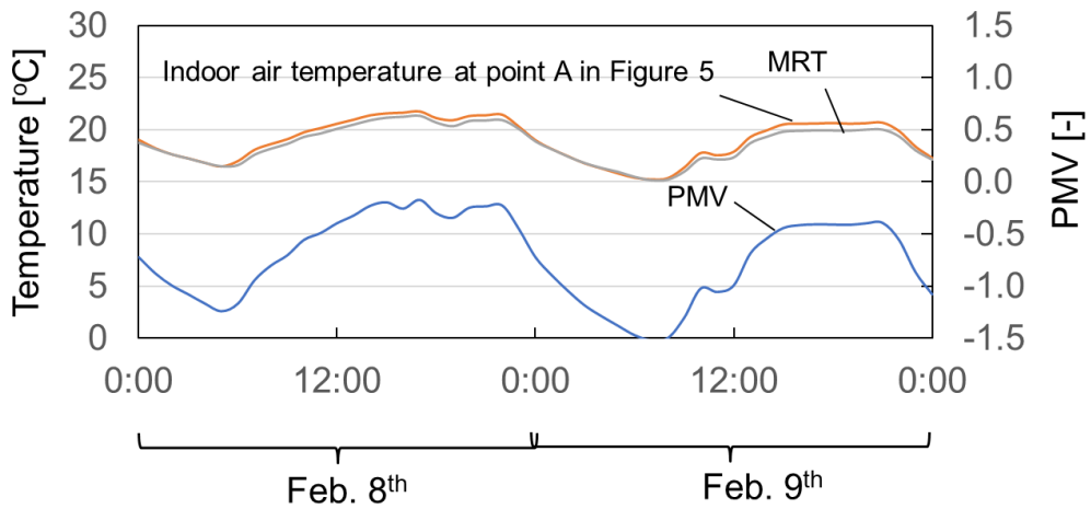
Fig. 9. Variations of indoor air temperature, MRT, and PMV at point A indicated in Figure 5 on February 8 th and 9 th in 2019
