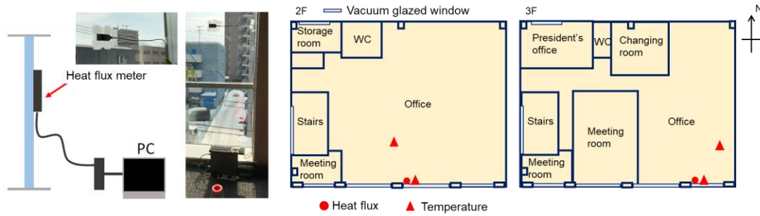
Fig. 6. (Left) Outlines and appearance of measuring heat flux, (Centre and Right) Arrangement of sensors to evaluate vacuum glazed windows.
