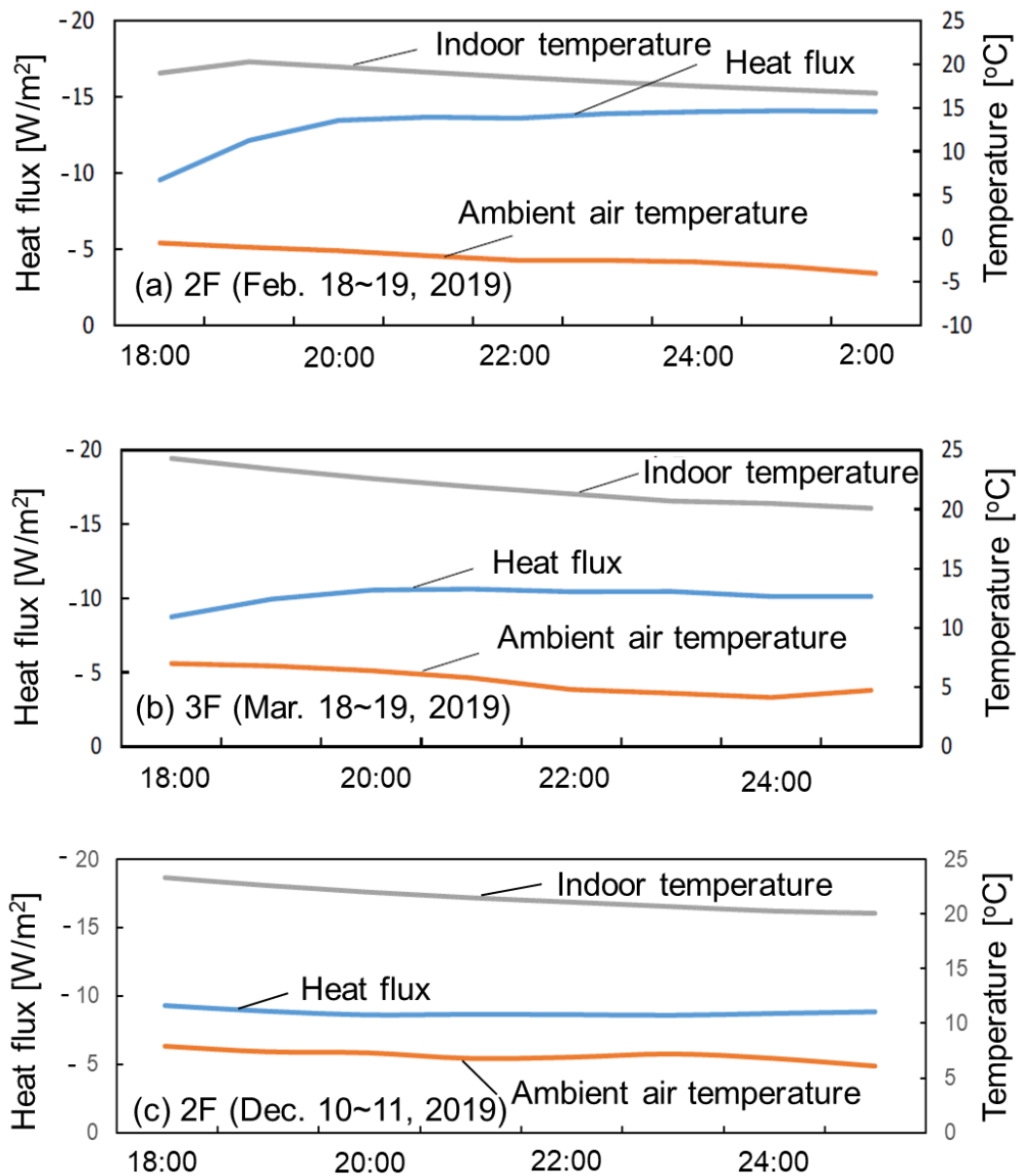
Fig. 11. Variations of heat flux, indoor air temperature, and ambient air temperature ((a) 2F (Feb. 18~19, 2019), (b) 3F (Mar. 18~19, 2019), (c) 2F (Dec. 10~11, 2019))
