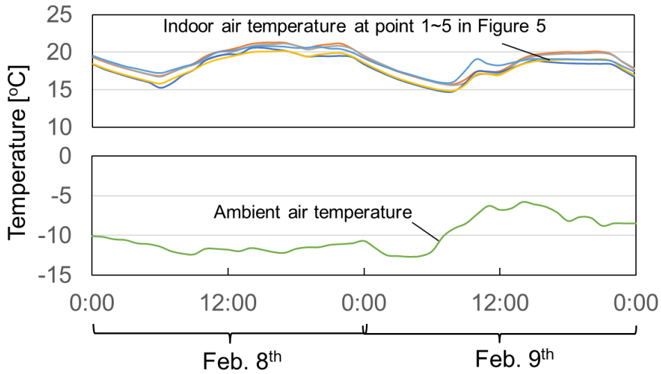
Fig. 8. Variations of indoor air temperature at point 1~5 indicated in Fig. 5 and ambient air temperature on February 8 th and 9 th in 2019
