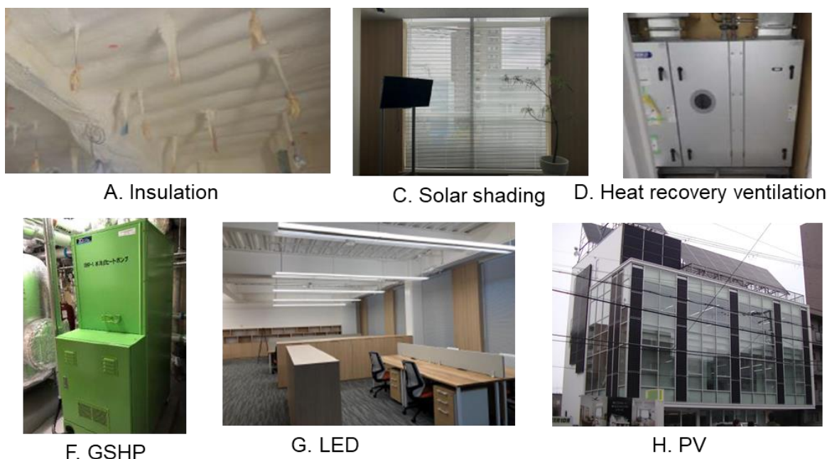
Fig. 3. Illustrates (a) internal insulation, (b) solar shading control blinds, (c) heat recovery ventilation system, (d) Ground Source Heat Pump (GSHP), (e) energy efficient LED lighting and (f) appearance of the installed PV system.
