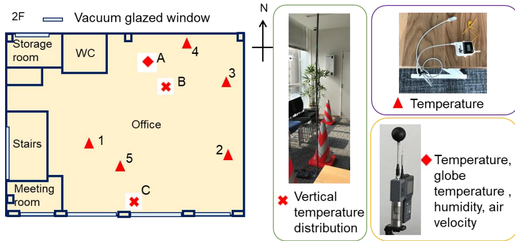
Fig. 5. (Left) Arrangement of sensors to evaluate thermal environment, (Right) Appearance of sensors installed in the office building
