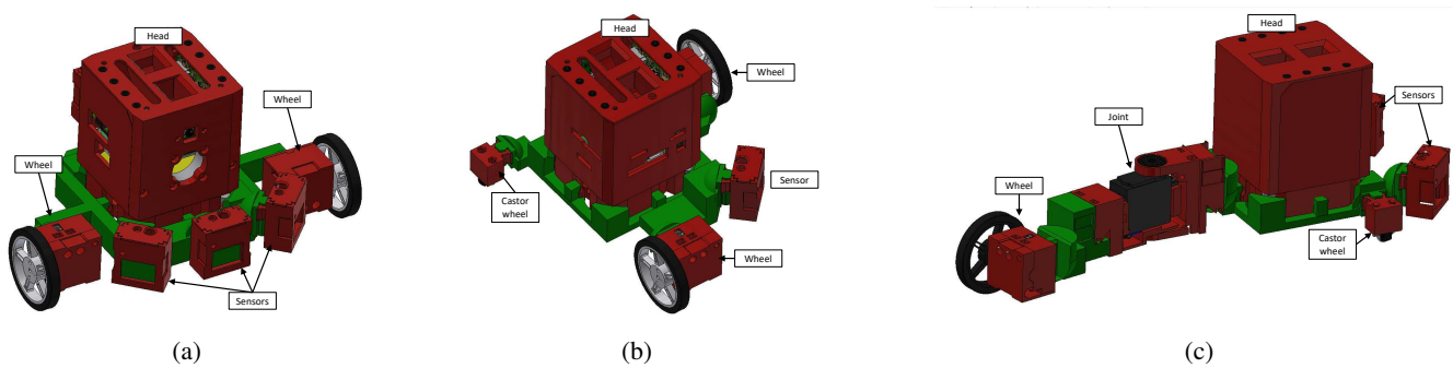
Fig. 10: Example body plans, designed by hand to demonstrate a range of possible robots for use in testing the physical assembly process and the simulation environment. (a) is the ARE-puck , which is symmetrical and designed to be easy to control, (b) the Potato which is similar but asymmetrical to add some complexity, and (c) the Tricycle which requires control of a joint and a wheel.
