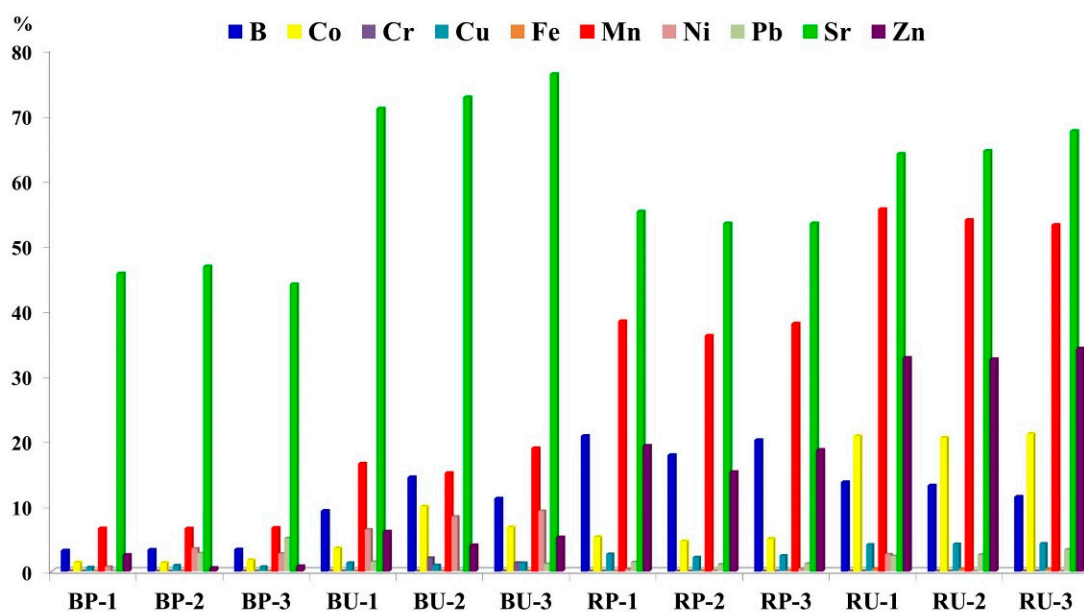
Figure 3. Mobility factor (%) for selected elements after modified BCR in studied urban soils (i.e., polluted- BP and RP, and unpolluted sites-BU and RU, in Belgrade and Reading).
