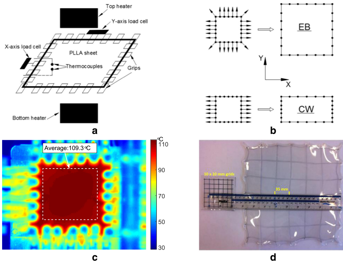
Fig. 4 Biaxial stretch testing, (a) machine arrangement; (b) deformation mode (EB: equal biaxial, CW: constant-width); (c) thermal images of a testing sample at 110 °C [38]; (d) a testing sample marked with grid lines before and after stretch [38]
