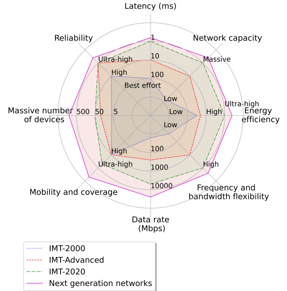
Figure 2: Requirements of KPIs [10] for IMT-2000, IMT-Advance, IMT-2020 and the future networks.
