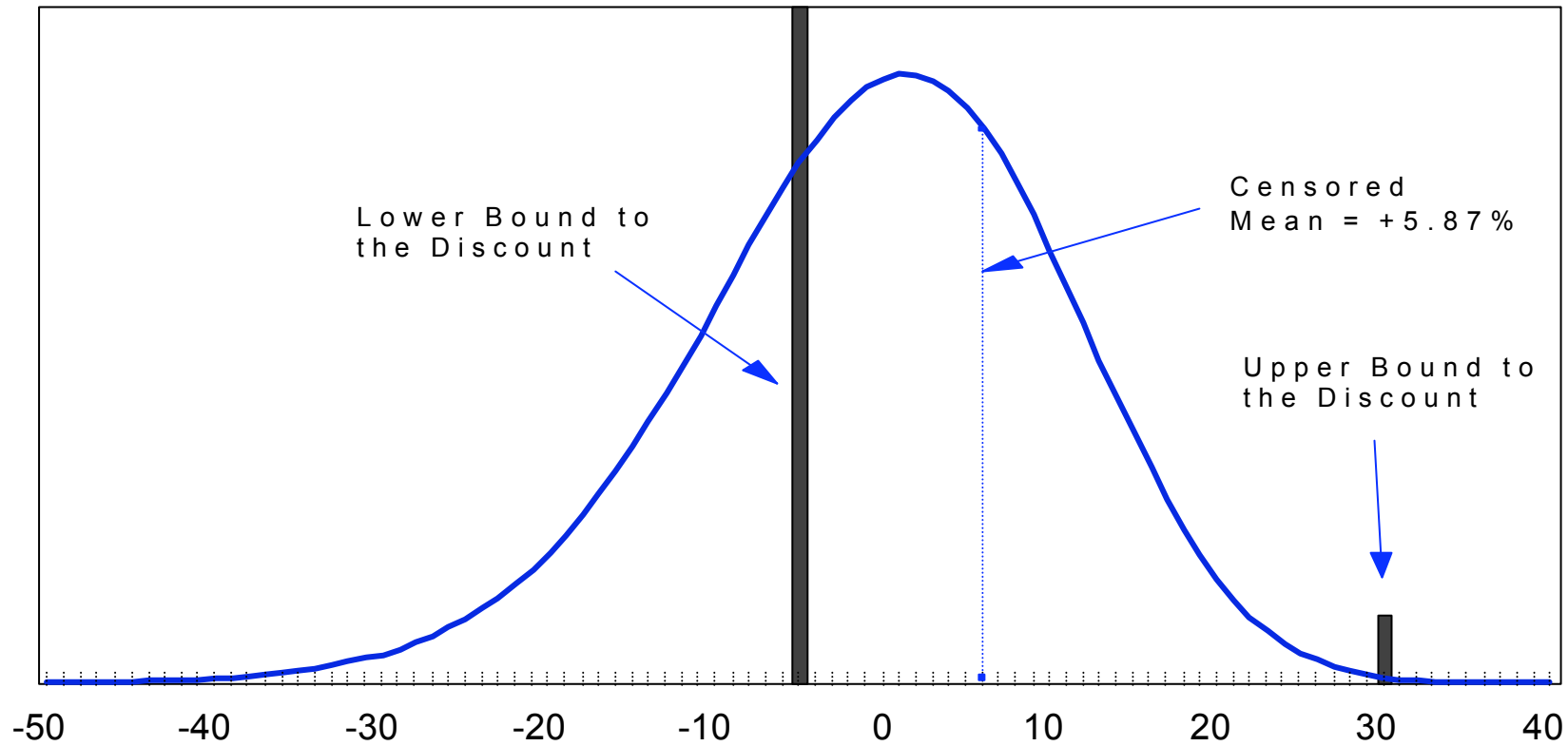
Figure 2. The censored distribution of the discount. The figure demonstrates how arbitrages may censor the distribution of the discount. A lognormal distribution with a mean of zero and standard deviation of 11.2 percent is plotted, upon which are imposed an upper bound of 30 percent and a lower bound of minus five percent. The result is that the mean of the distribution changes from zero to +5.87 percent.
