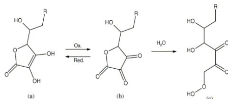
Fig. 8: Degradation reaction of AP
