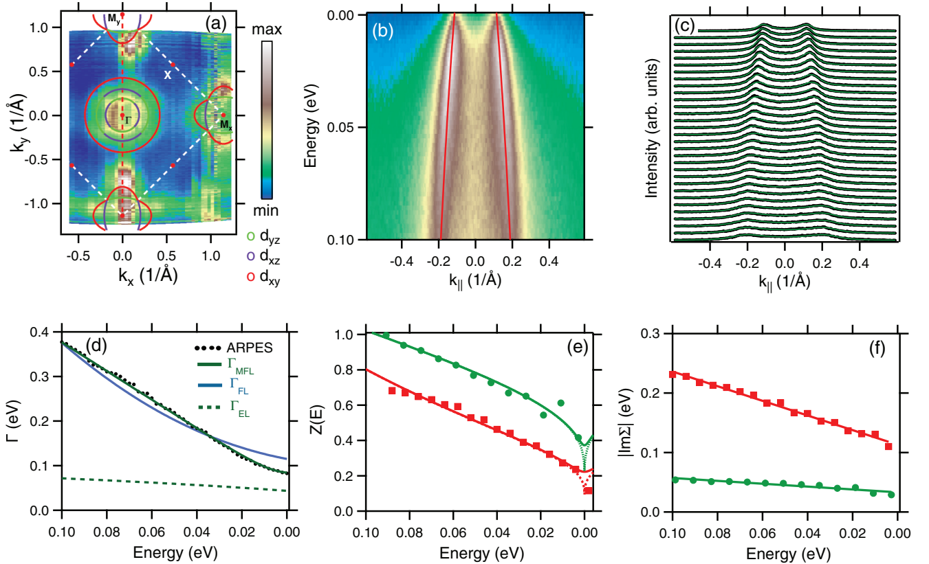
FIG. 1. ARPES data of optimally hole-doped K_{0.4}Ba_{0.6}Fe_2As_2 in the normal state at T = 50 K measured with h\nu = 75 eV vertically polarized photons. (a) Fermi surface derived from ARPES spectral weight near the Fermi level. The data are overlaid with a schematic plot of the Fermi surface of the three hole pockets near \Gamma and two electron pockets near the M points. The predominant orbital character is indicated by colors. (b) Experimental energy-momentum distribution map, measured along the red dashed line in (a). Red line: fitted dispersion. (c) Waterfall plot of the MDCs (black points) together with a least-squares fit (green lines). Uppermost spectrum E = E_F , lowest spectrum E = 0.12 eV. (d) Experimental scattering rates \Gamma(E, T = 50 K) (black points) as a function of energy derived from the least-squares fit of the intensity distribution. Green line: fit with a theoretical non-Fermi liquid model (see text). Dashed green line: estimated contribution from elastic scattering. Blue line: fit with a Fermi liquid behavior. (e) Renormalization function Z(E) derived from ARPES data (red squares). Solid red line: fit to a function given in Eq. (3). The results are compared with analogous data from BaCr_2As_2 (green points, solid green line). The dotted lines are extrapolations of the fit curves to zero temperature. (f) Imaginary part of the self energy \text{Im}\Sigma(E) derived from our experimental values \Gamma(E) and Z(E) using the relation \Gamma(E) = -2Z(E)\text{Im}\Sigma(E) (red squares). Solid red line: fit to a linear energy dependence. The results are compared with analogous data from BaCr_2As_2 (green points, solid green line).
