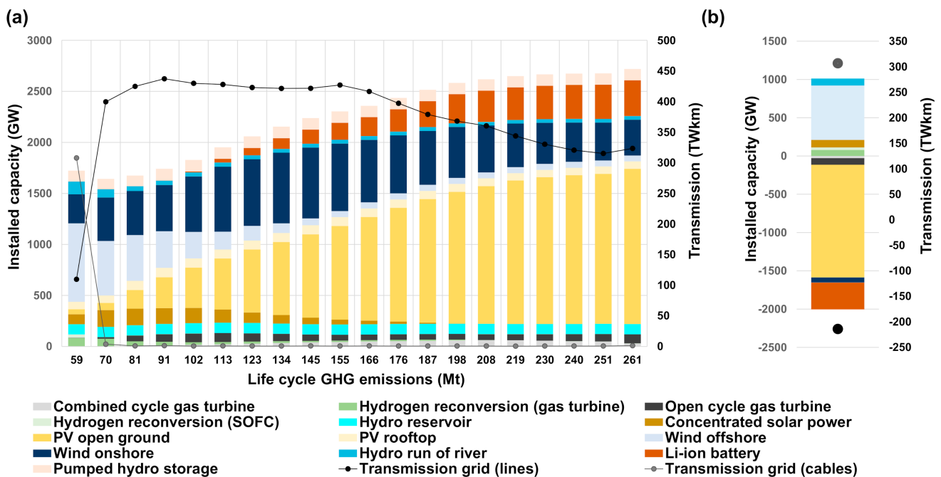
Figure 7. Power plant and power storage portfolio and transmission capacities in the EUNA region in case of a complete phase-out of nuclear power by 2050. Panel (a) shows the power plant and storage portfolio (left y -axis) and the grid installations (right y -axis) for each solution on the pareto front (Figure S1 (Supplementary Materials)). Panel (b) shows the technology specific differences between the cost-optimal solution and the least life cycle GHG emissions-intensive solution for both, power generation and storage capacities and grid. Technologies with less than a 1% share of capacity in any solution are not shown for the sake of clarity.
