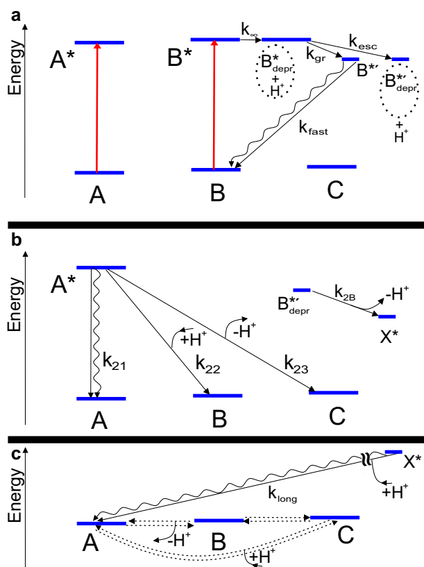
Fig. 17 Extended kinetic scheme of the photoreaction of PCB (as described in the text) after excitation with \lambda_{exc}=580 nm, divided in the time ranges of \tau_1 (a), \tau_2 (b) and \tau_3 , as well as for long time scales (both c). Red arrows indicate excitation; straight and wavy lines indicate radiationless and radiative transitions, respectively. Dotted arrows show thermally driven equilibrium reactions of the ground state species. a Assuming k_{fast} \gg k_{gr} , (k_{gr} + k_{esc})^{-1} = \tau_1 , k_{inf}^{-1} < 0.38 ps (system response time). b (k_{21} + k_{22} + k_{23})^{-1} = \tau_2 , (k_{2B})^{-1} is the time constant resulting from the biexponential fit of CA2. c The apparent time constant \tau_3 is determined by the rate constants governing the thermal equilibration between excess population of B and C with A. For more information cf. main text
