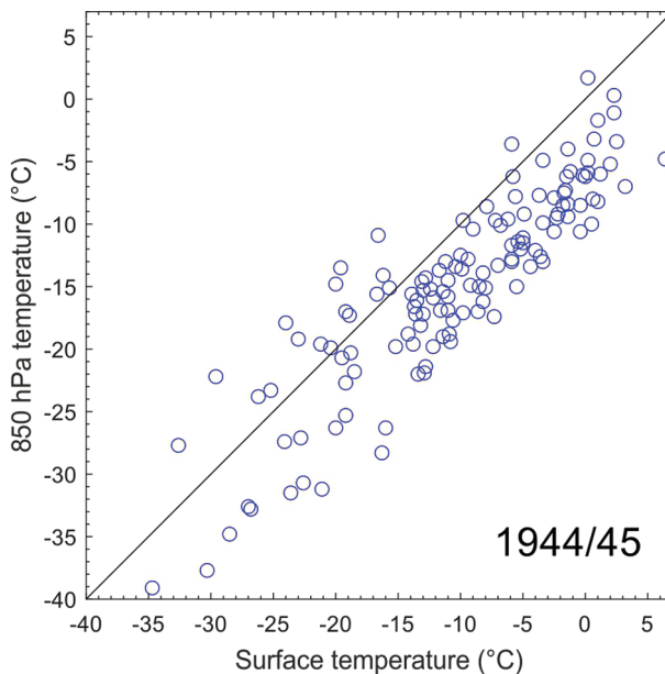
Fig. 5 Rijpfjorden 1944/45 surface temperatures against 850 hPa temperatures from radiosonde launches. Only a few of the low surface temperatures in winter are associated with boundary-layer inversions. Generally, surface temperatures are strongly correlated with 850 hPa temperatures ( R^2 = 0.79 ).
