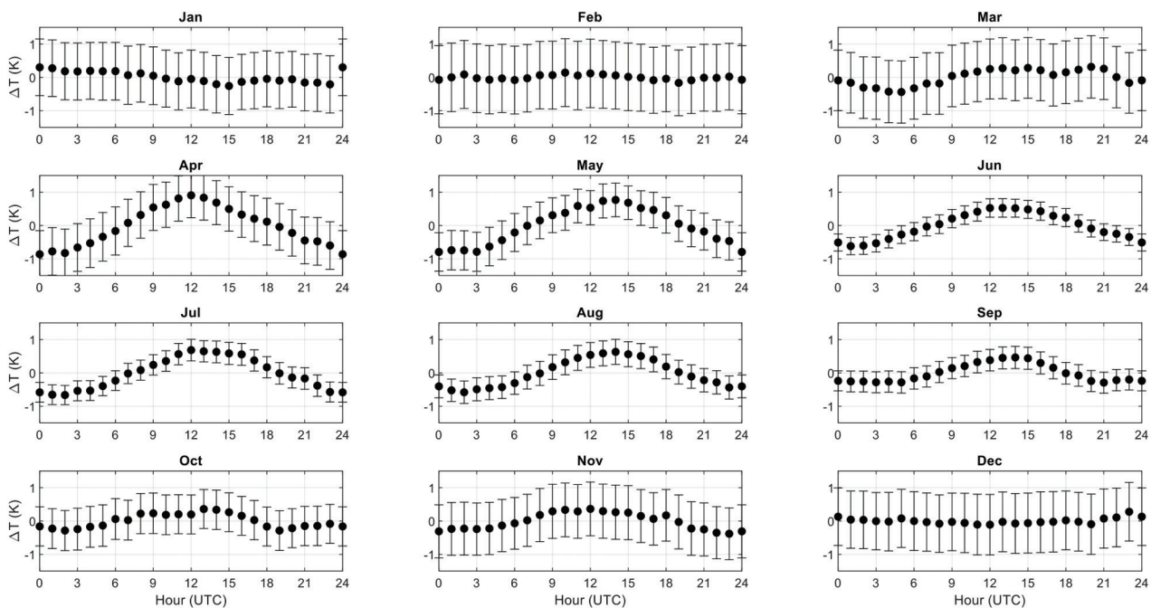
Fig. 3 Diurnal temperature variation (deviation from daily means) at Rijpfjorden for 2014–16. Error bars denote one standard error.
