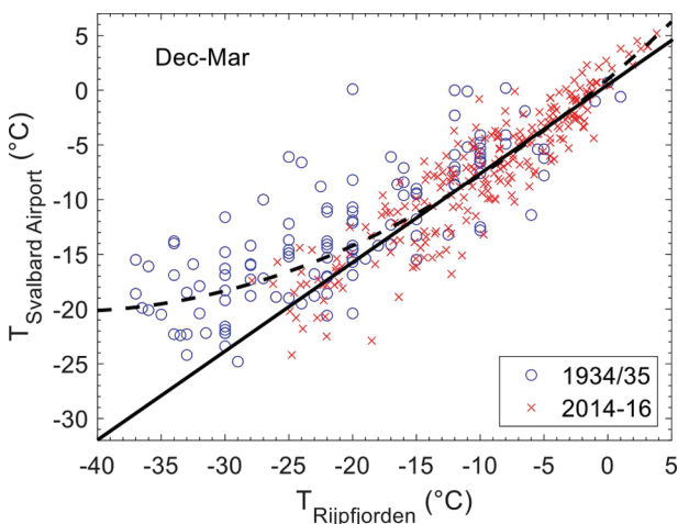
Fig. 4 Relation between Rijpfjorden and Svalbard Airport temperatures during the winter months December to March. The dashed line is a second-order polynomial fit through all data points (1934/35 and 2014–16), and the solid line represents the linear fit to the 2014–16 data only.
