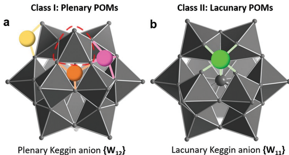
Figure 3. Classification of POM-SACs together with an illustration of prototypical binding sites and coordination modes. a) Class I POM-SACs: SAC binding sites in the plenary Keggin anion [X_{M_{12}O_{40}}]^{n-} (= {W12}). b) Class II POM-SACs, highlighting the additional metal binding site in a lacunary Keggin anion [X_{M_{11}O_{39}}]^{m-} (= {W11}). [52] SAC sites indicated in a) can be described as surface sites, whereas the SAC site in b) results from metal substitution within the Keggin metal oxide framework. Note that {W11} is formed by hydrolytic removal of a “W = O” group from {W12} (marked in a) by a red dashed circle).
