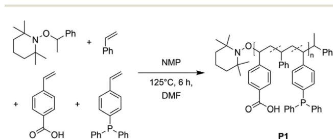
Scheme 1 Synthesis of the terpolymer P1 by nitroxide-mediated radical polymerization of styrene, 4-vinylbenzoic acid and diphenyl(4-vinylphenyl)phosphine. The alkoxyamine was used as initiating material.
