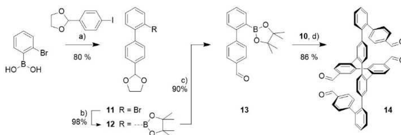
Scheme 4. Synthesis of the biphenyl building-block 13 and its merger with the ortho -tetraphenylene 10 forming the advanced precursor 14 . a) K_2CO_3 , Pd(PPh_3)_2Cl_2 (cat.), THF/MeOH (4:1), reflux, 4 h (argon); b) n BuLi then i PrB pinv , THF, -78 °C to RT, 1.5 h (argon); c) PTSA, acetone/water (10:1), RT, overnight; d) K_3PO_4 \cdot H_2O , Pd(PPh_3)_4 , dioxane/water (5:1), reflux, overnight (argon).
