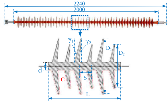
FIGURE 2. FXBW-220/100 composite insulator and simulation selected section.
