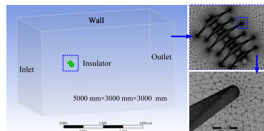
FIGURE 3. Simulation domain and mesh.
