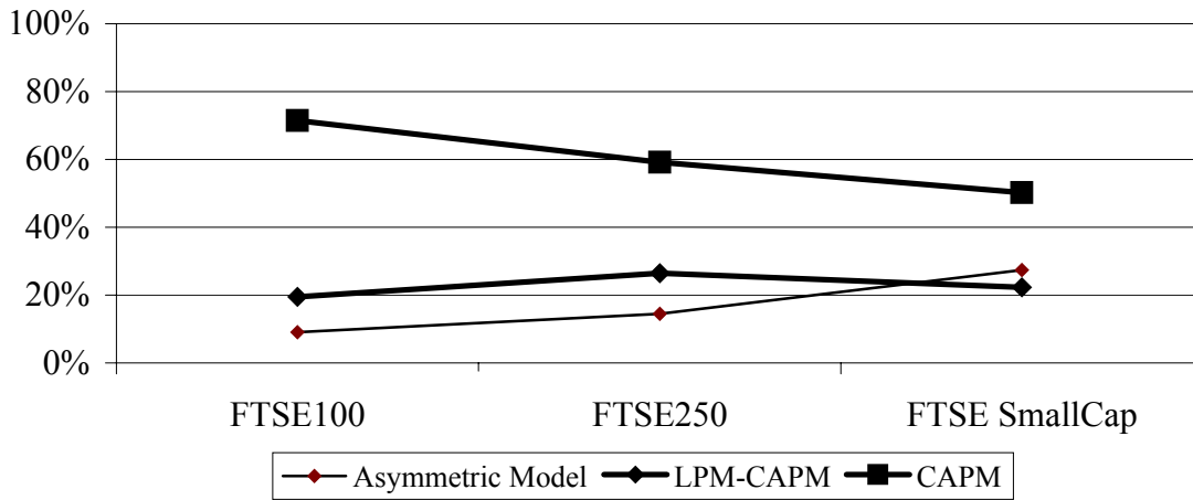
Figure 1A Percent of the Choice of the Three Models for Daily Returns Obtained with MG Distribution
