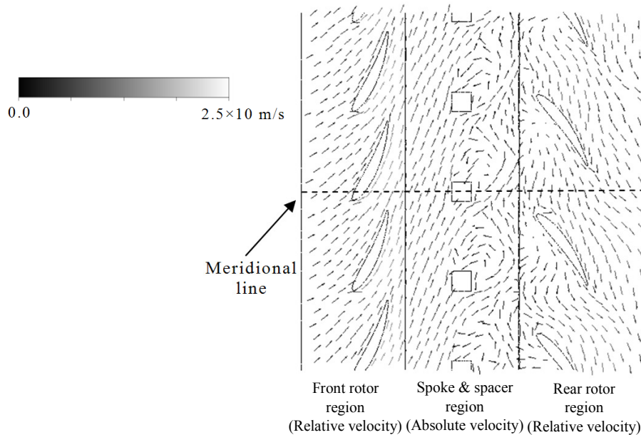
(b) r/r_c=0.58, \theta_f=0^\circ, \theta_r=-30^\circ
