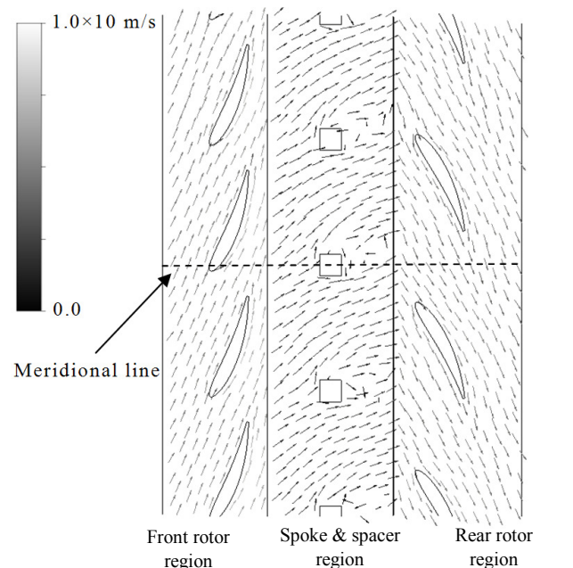
Figure.8 Velocity vectors
