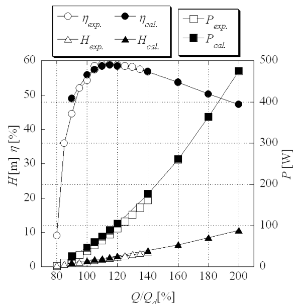
Figure.6 Performance curves
