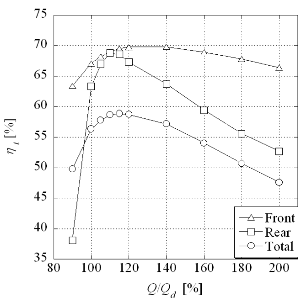
Figure.7 Total pressure efficiency
