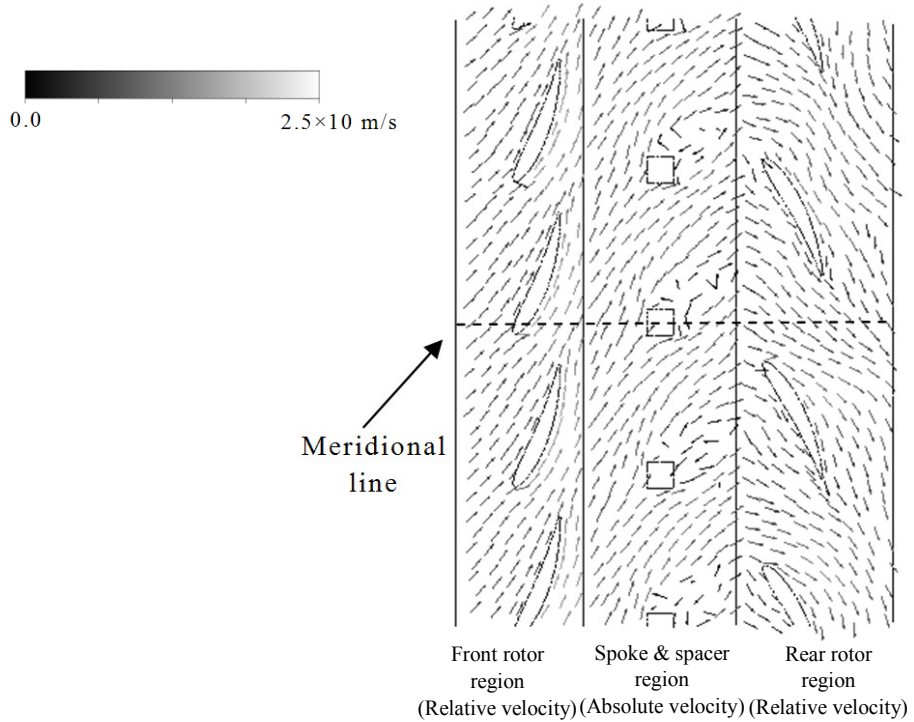
(a) r/r_c=0.74, \theta_f=0^\circ, \theta_r=-30^\circ
