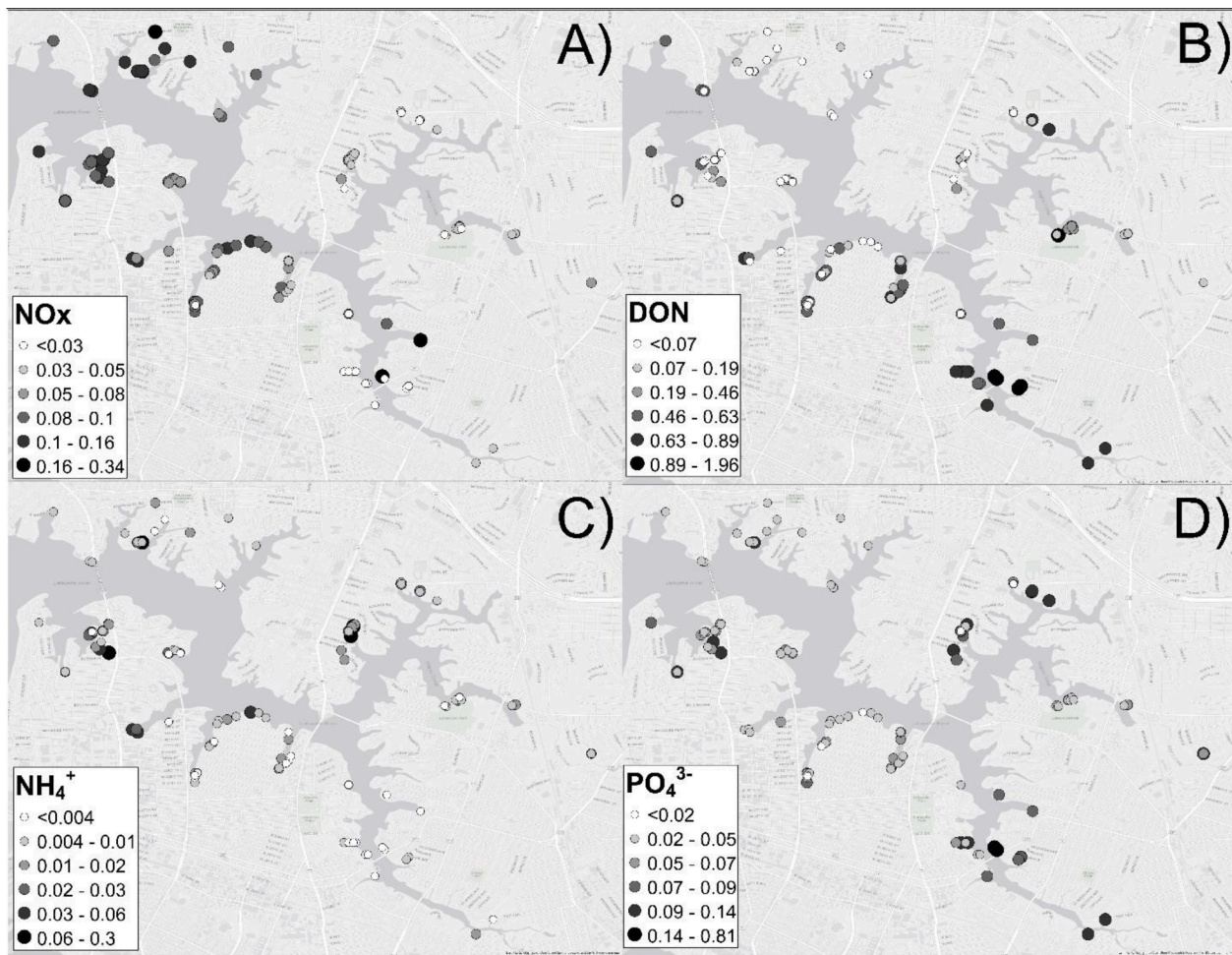
Fig. 2. The concentration of (A) NOx-N, (B) DON-N, and (C) NH 4 + -N, and (D) PO 4 3- -P, all in mg L -1 , in floodwater samples collected by citizen-science volunteers during the perigeal spring tide of November 5, 2017.
