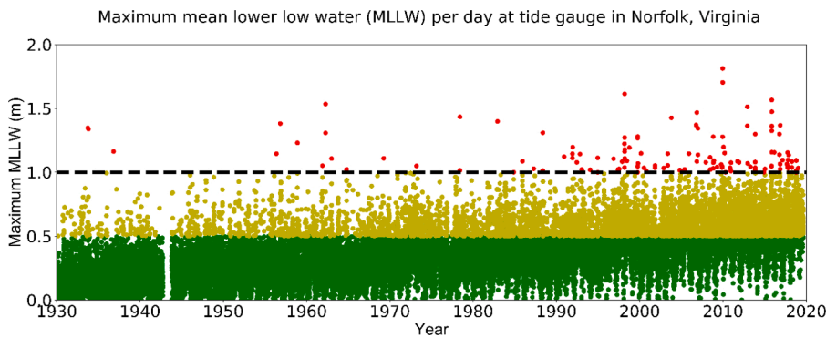
Fig. 5. Maximum water levels measured between 1930 and 2019 at the Sewells Point station, Norfolk, VA. Green dots (MLLW <0.5 m) are considered a ‘no flooding scenario’, while yellow (MLLW 0.5 - 1 m) and red dots (MLLW >1 m) are water levels that produce flooding in this region as exemplified in Fig. 1. The dotted line shows the water level during our sampling campaign. Data source: NOAA’s Tides & Currents ( https://tidesandcurrents.noaa.gov ) (For interpretation of the references to color in this figure legend, the reader is referred to the web version of this article.).
