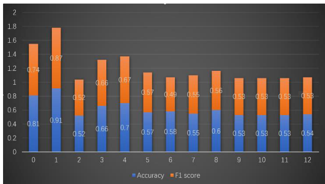
FIGURE 7. Robustness test.
