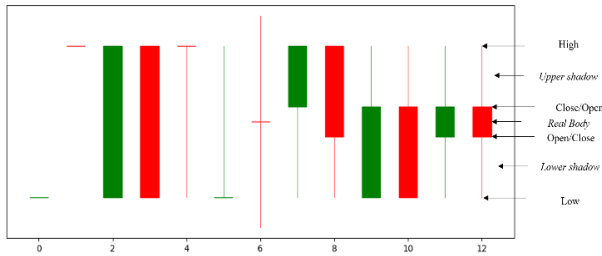
FIGURE 3. Candlestick patterns.
