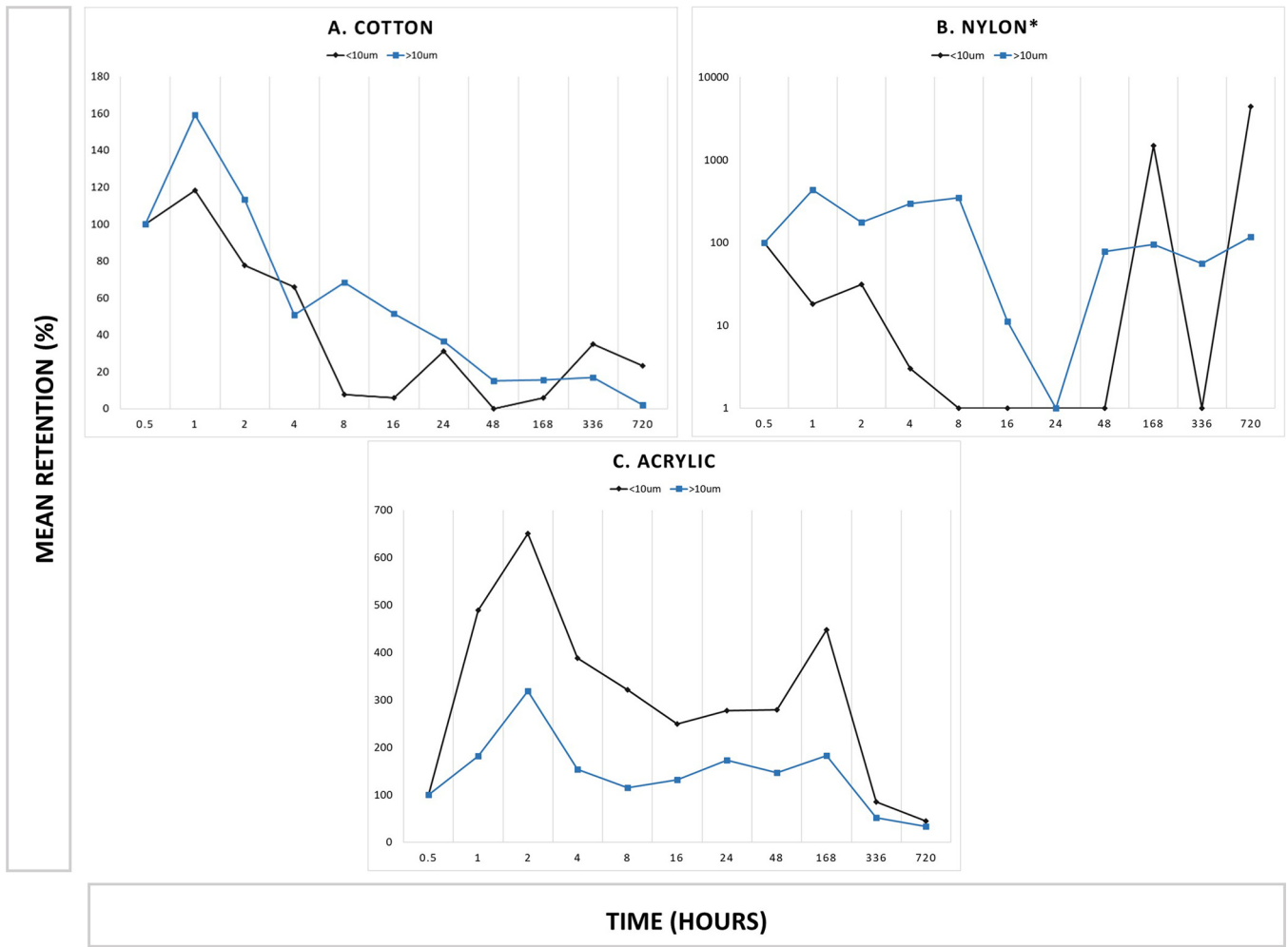
Fig. 3. a-c: The mean retention (%) of diatoms less than (<) and greater than (>) 10 µm in size on the three clothing materials tested following up to one month (720 h) of wear in the winter (n = 3).
