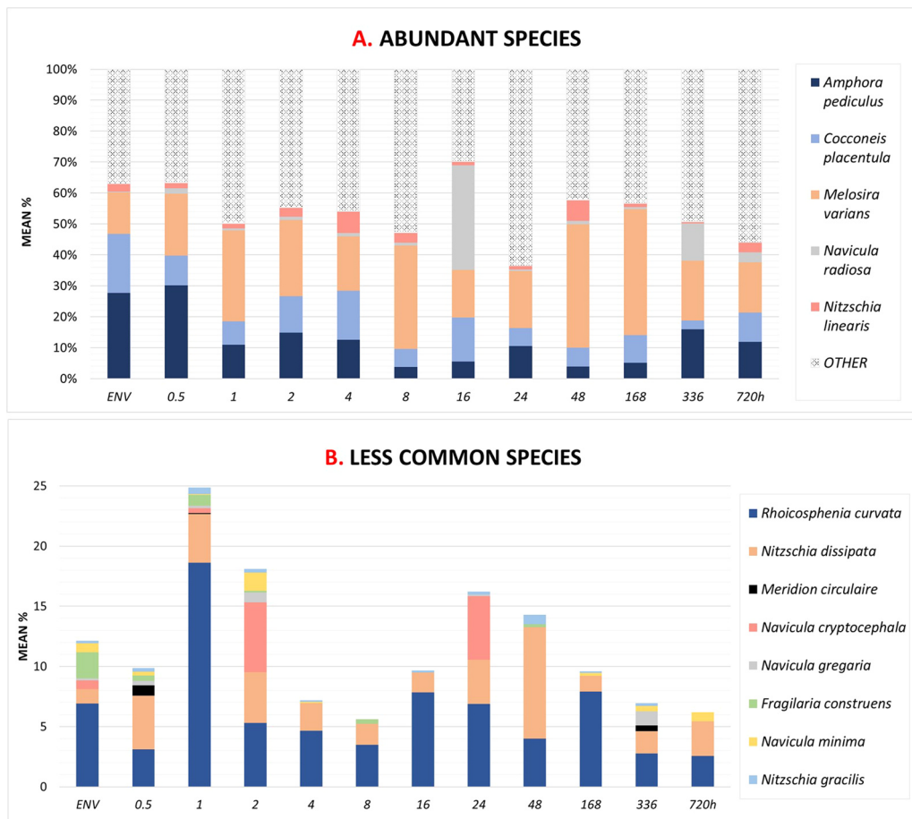
Fig. 9. The relative abundance (%) of the five most abundant (A) and eight relatively less common (B) environmental control diatom species in the winter environmental and persistence samples. Overall values (per time since wear interval) are presented (n = 9).
