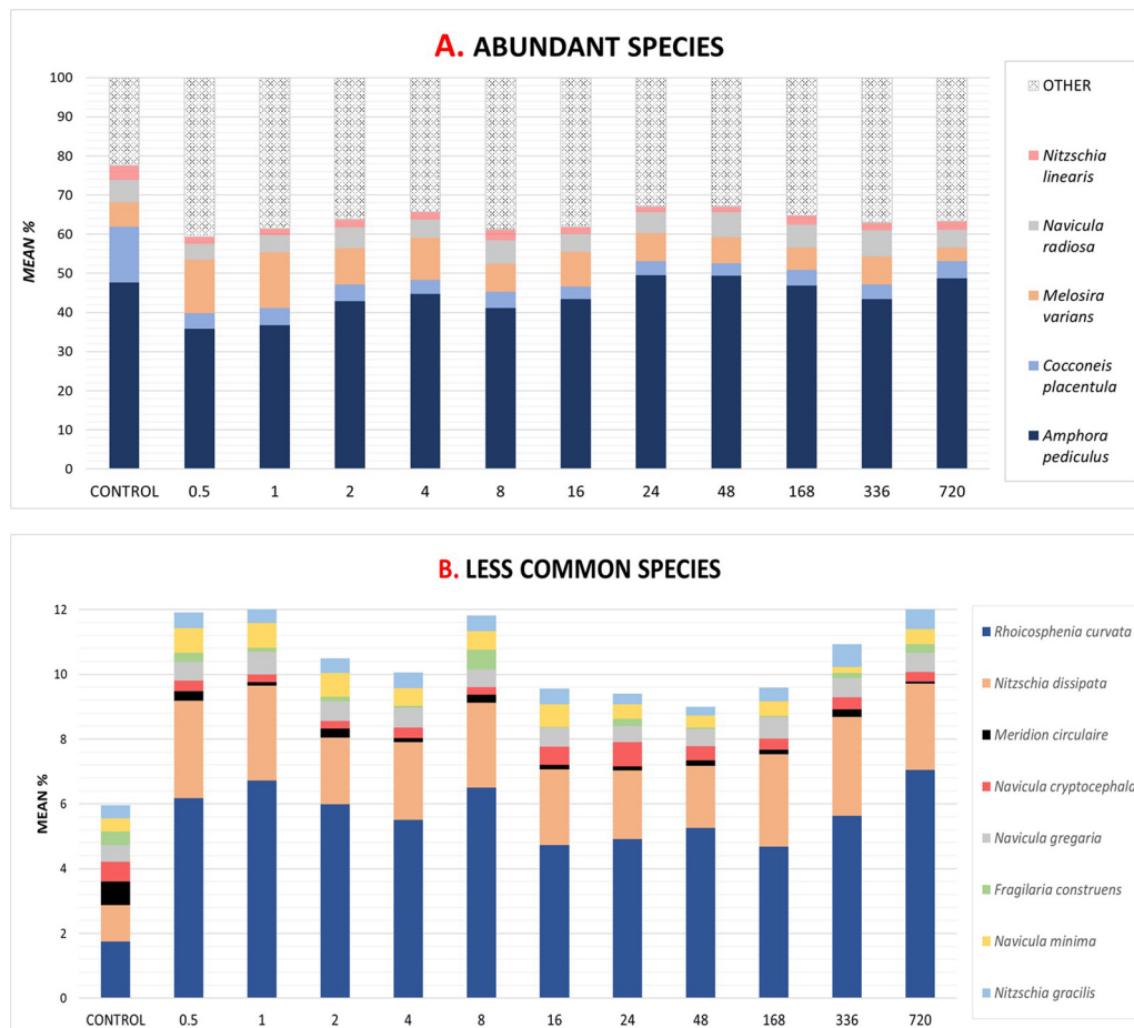
Fig. 8. The relative abundance (%) of the five most abundant (A) and eight relatively less common (B) environmental control diatom species in the spring environmental and persistence samples. Overall values (per time since wear interval) are presented ( n=9 ), with trends for each clothing type included in Supplementary Figs. 8 and 9 .
