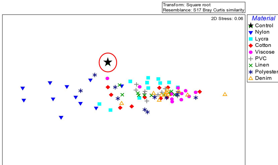
Fig. 4. NMDS plot of the mean diatom species assemblage in the spring environmental (*) and all clothing persistence samples, based on Bray-Curtis matrix. Data points that are closer to each other represent samples with a more similar assemblage. Summary of ANOSIM data, including two-way samples comparisons, is presented in Supplementary Table 2 and Supplementary Fig. 3 .
