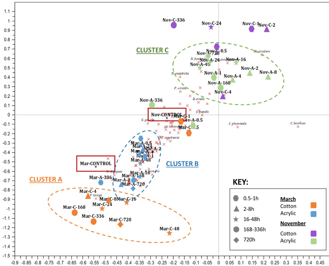
Fig. 6. Canonical correspondence analysis plot highlighting the variability between the seasonal environmental controls and most acrylic and cotton persistence samples. Data points that are closer to each other represent samples with a more similar diatom species assemblage. The 8–720 h winter cotton and all nylon samples demonstrated greater variability and are presented in Supplementary Figs. 4 and 5.
