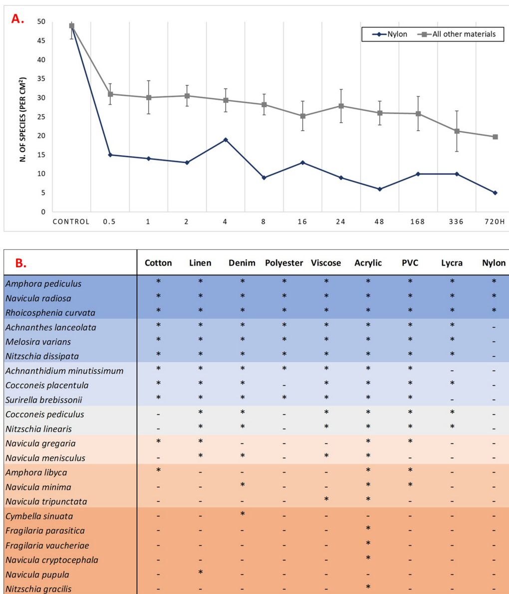
Fig. 5. The retention of environmental control sample taxa identified in each spring persistence sample (A) and the range of diatom species consistently identified (*) from 0 to 720 h of wear in one or more clothing types in spring (B). All other source environment species were retrieved less frequently or were absent from the spring persistence samples [Supplementary Datafile].
