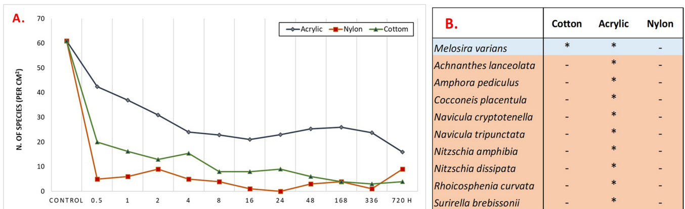
Fig. 7. The retention of environmental control sample taxa identified in each winter persistence sample (A) and the range of diatom species consistently identified (*) from 0 to 720 h of wear in one or more clothing types in winter (B). All other source environment species were retrieved less frequently or were absent from the spring persistence samples [Supplementary Datafile].
