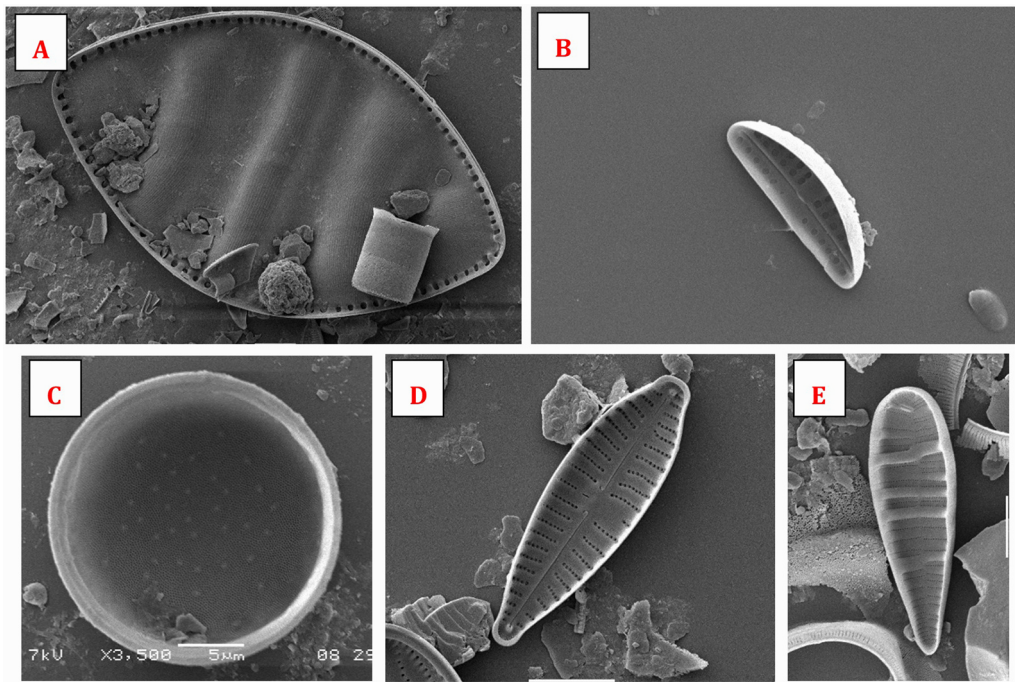
Fig. 1. SEM micrographs of selected diatom species belonging to the different morphological groups (size and shape) chosen for comparison: a) Size > 10 \mu\text{m} : Cymatopleura elliptica (x1000 mag.); b) Size < 10 \mu\text{m} : Amphora pediculus (x5000 mag.); c) Shape – centric: Melosira varians (x3500 mag.); d) Shape – raphid pennate: Gomphonema angustatum (x4500mag.); e) Shape – araphid pennate: Meridion circulare (x4300mag.). All images were taken using Jeol JSM-6480LV.
