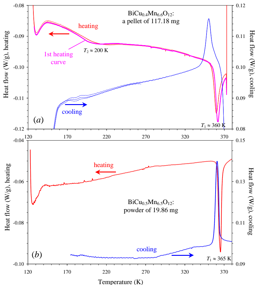
Figure 5. DSC curves of (a) \text{BiCu}_{0.4}\text{Mn}_{6.6}\text{O}_{12} (three runs) and (b) \text{BiCu}_{0.5}\text{Mn}_{6.5}\text{O}_{12} (one run) on heating (left-hand axes) and cooling (right-hand axes) at 10 K/min. Note that the heating and cooling difference scale ranges are the same.
