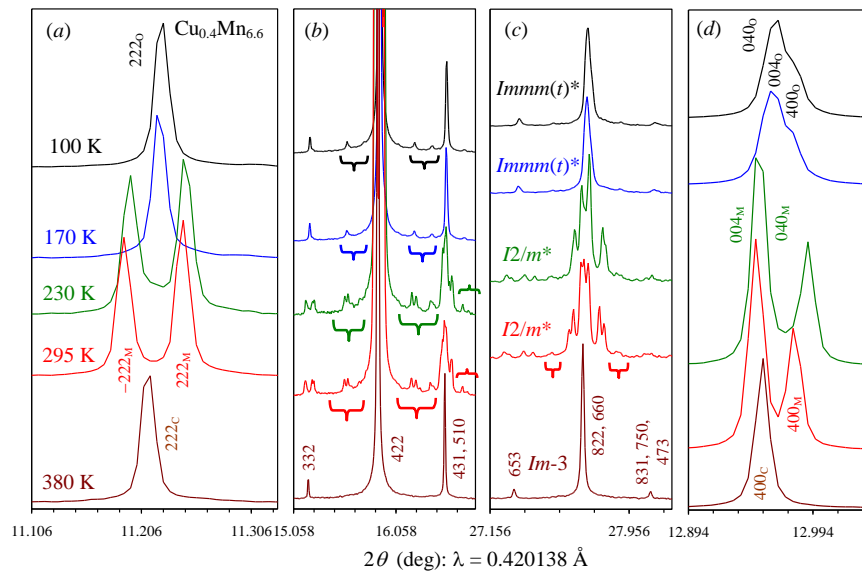
Figure 6. Fragments of synchrotron XRPD data (BL02B2) of \text{BiCu}_{0.4}\text{Mn}_{6.6}\text{O}_{12} in different 2\theta regions at T = 100 K, 170 K, 230 K, 295 K, and 380 K. Some reflection indexes for the cubic phase (without notations and with the C notation), the monoclinic (M) phase and the orthorhombic (O) phase are given. Braces show incommensurately modulated reflections.
