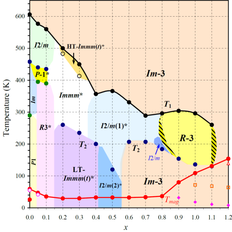
Figure 16. Composition-temperature phase diagram of \text{BiCu}_x\text{Mn}_{7-x}\text{O}_{12} solid solutions for 0 \leq x \leq 1.2 . Stars indicate the presence of additional incommensurately modulated reflections, t stands for pseudo-tetragonal. Shaded regions show mixed-phase regions. Magnetic transition temperatures ( T_{\text{mag}} : red and pink symbols) are also plotted for completeness (but detailed magnetic studies will be reported elsewhere). T_1 denotes a phase transition from the high-temperature cubic Im-3 phase. T_2 denotes the lowest temperature structural phase transition.
