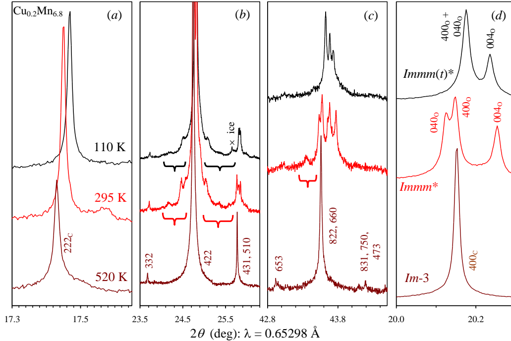
Figure 2. Fragments of synchrotron XRPD data (BL15XU) of \text{BiCu}_{0.2}\text{Mn}_{6.8}\text{O}_{12} in different 2\theta regions at T = 110 K, 295 K, and 520 K. Some reflection indexes for the cubic phase (without notations and with the C notation) and the orthorhombic (O) phase are given. A cross marks a possible reflection from ice. Braces show modulated reflections.
