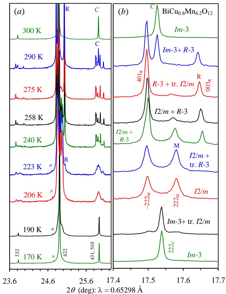
Figure 14. Fragments of synchrotron XRPD data (BL15XU) of \text{BiCu}_{0.8}\text{Mn}_{6.2}\text{O}_{12} in different 2\theta regions at different temperatures. Some reflection indexes for the cubic phase (without notations and with the C notation), the monoclinic (M) phase, and the R -3 phase (R) are given. Crosses mark a reflection from ice. tr.: trace.
