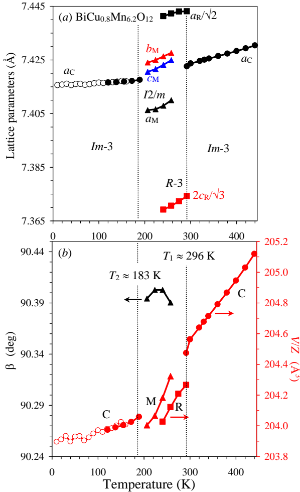
Figure 15. Temperature dependence of (a) the lattice parameters and (b) monoclinic \beta angle (left-hand axis) and the unit-cell volume ( V/Z ) (right-hand axis) in \text{BiCu}_{0.8}\text{Mn}_{6.2}\text{O}_{12} from laboratory XRPD data (open circles; 10-160 K) and synchrotron XRPD data (filled symbols; 120-440 K). All measurements were performed on heating. C: cubic, M: monoclinic, R: R-3 . \alpha_V = 1.93(13) \times 10^{-5} in the HT C phase, \alpha_V = 2.3(6) \times 10^{-5} in the R phase, \alpha_V = 3(1) \times 10^{-5} in the M phase and \alpha_V = 6(3) \times 10^{-6} at 120-180 K in the LT C phase.
