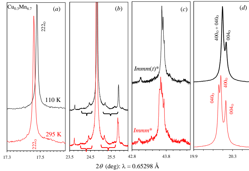
Figure 3. Fragments of synchrotron XRPD data (BL15XU) of \text{BiCu}_{0.3}\text{Mn}_{6.7}\text{O}_{12} in different 2\theta regions at T = 110 K and 295 K. Some reflection indexes for the orthorhombic (O) phase are given. Braces show modulated reflections.
