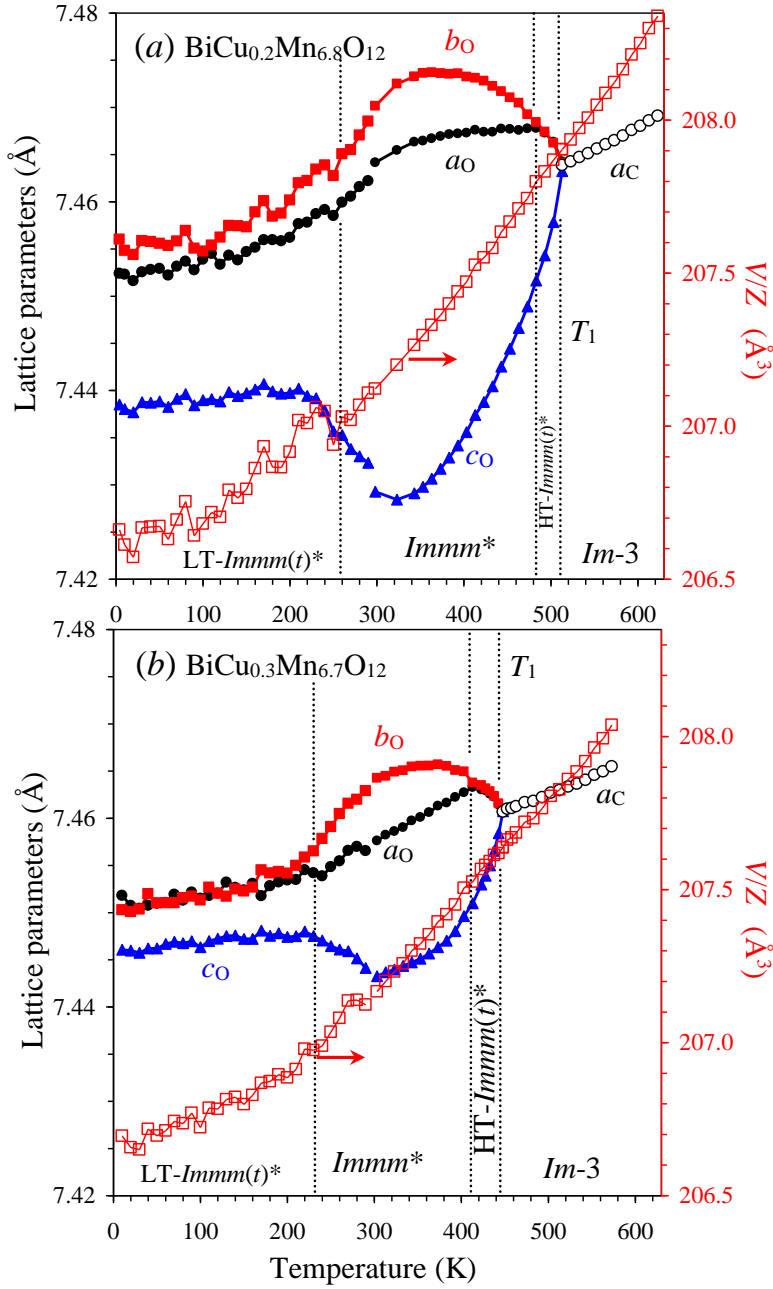
Figure 4. Temperature dependence of the lattice parameters (left-hand axes) and the unit-cell volume ( V/Z ) (right-hand axes) in (a) \text{BiCu}_{0.2}\text{Mn}_{6.8}\text{O}_{12} and (b) \text{BiCu}_{0.3}\text{Mn}_{6.7}\text{O}_{12} from laboratory XRPD data. All measurements are performed on heating. C: cubic, O: orthorhombic, t : pseudo-tetragonal. HT: high-temperature, LT: low-temperature. Stars indicate the presence of additional incommensurately modulated reflections. \alpha_V = 1.8(4) \times 10^{-5} at 300-610 K for x = 0.2 , \alpha_V = 1.5(5) \times 10^{-5} at 300-560 K and \alpha_V \sim 5 \times 10^{-6} at 10-210 K for x = 0.3 .
