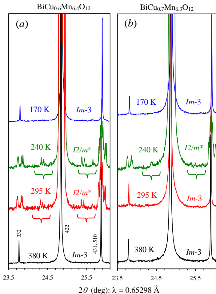
Figure 12. Fragments of synchrotron XRPD data (BL15XU) of (a) \text{BiCu}_{0.6}\text{Mn}_{6.4}\text{O}_{12} and (b) \text{BiCu}_{0.7}\text{Mn}_{6.3}\text{O}_{12} in a 2\theta region of 23.5–26.1 deg at T = 170 K, 240 K, 295 K, and 380 K. Some reflection indexes for the cubic phase (without notations) are given. Braces show modulated reflections.
