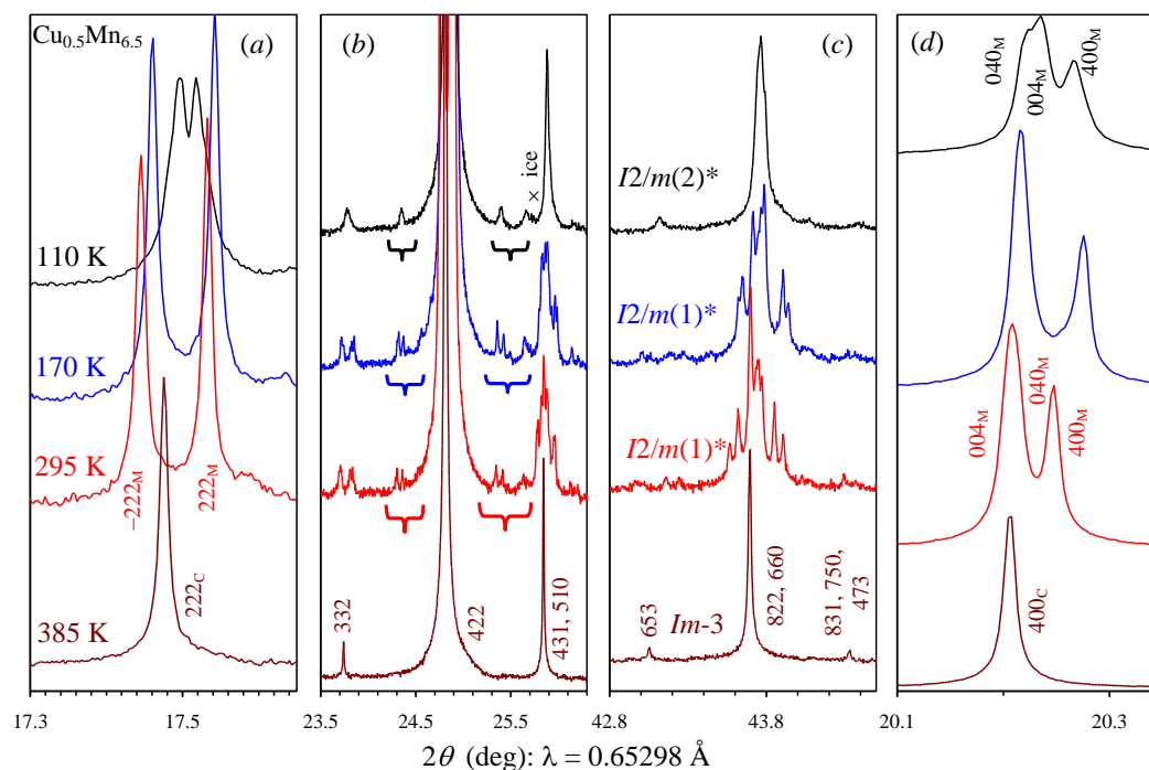
Figure 8. Fragments of synchrotron XRPD data (BL15XU) of BiCu 0.5 Mn 6.5 O 12 in different 2\theta regions at T = 110 K, 170 K, 295 K, and 385 K. Some reflection indexes for the cubic phase (without notations and with the C notation) and the monoclinic (M) phase are given. A cross marks a possible reflection from ice. Braces show incommensurately modulated reflections.
