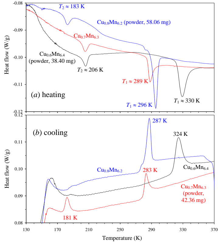
Figure 11. DSC curves of \text{BiCu}_{0.6}\text{Mn}_{6.4}\text{O}_{12} (black), \text{BiCu}_{0.7}\text{Mn}_{6.3}\text{O}_{12} (red), and \text{BiCu}_{0.8}\text{Mn}_{6.2}\text{O}_{12} (blue) on (a) heating and (b) cooling at 10 K/min. Note the heating and cooling difference scale ranges are the same.
