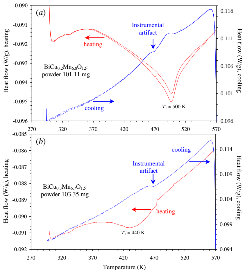
Figure 1. DSC curves of (a) \text{BiCu}_{0.2}\text{Mn}_{6.8}\text{O}_{12} (two runs) and (b) \text{BiCu}_{0.3}\text{Mn}_{6.7}\text{O}_{12} (one run) on heating (left-hand axes) and cooling (right-hand axes) at 10 K/min. Note the heating and cooling difference scale ranges are different. Small bumps near 470 K on cooling curves are instrumental artifacts.
