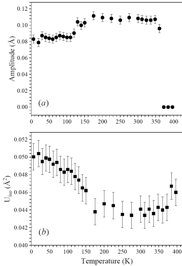
Figure 10. Temperature dependence of (a) the average amplitude of the Jahn-Teller distortions for two octahedral sites (Mn4 and Mn5) and (b) the atomic displacement parameter of the Bi site in the ideal (0, 0, 0) positions in BiCu 0.5 Mn 6.5 O 12 from neutron diffraction data.
