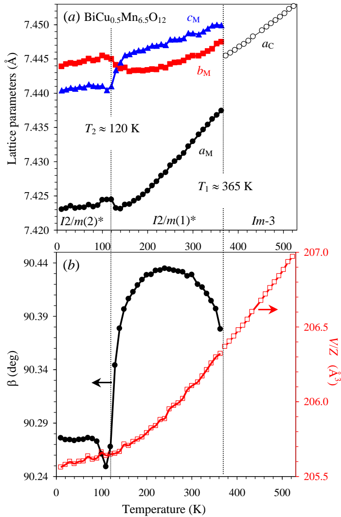
Figure 9. Temperature dependence of (a) the lattice parameters and (b) monoclinic \beta angle (left-hand axis) and the unit-cell volume ( V/Z ) (right-hand axis) in \text{BiCu}_{0.5}\text{Mn}_{6.5}\text{O}_{12} from laboratory XRPD data. Measurements were performed on heating. C: cubic, M: monoclinic. Stars indicate the presence of additional incommensurately modulated reflections. \alpha_V = 2.0(3) \times 10^{-5} at 370-510 K in the C phase and \alpha_V \sim 5 \times 10^{-6} at 10-100 K in the M phase.
