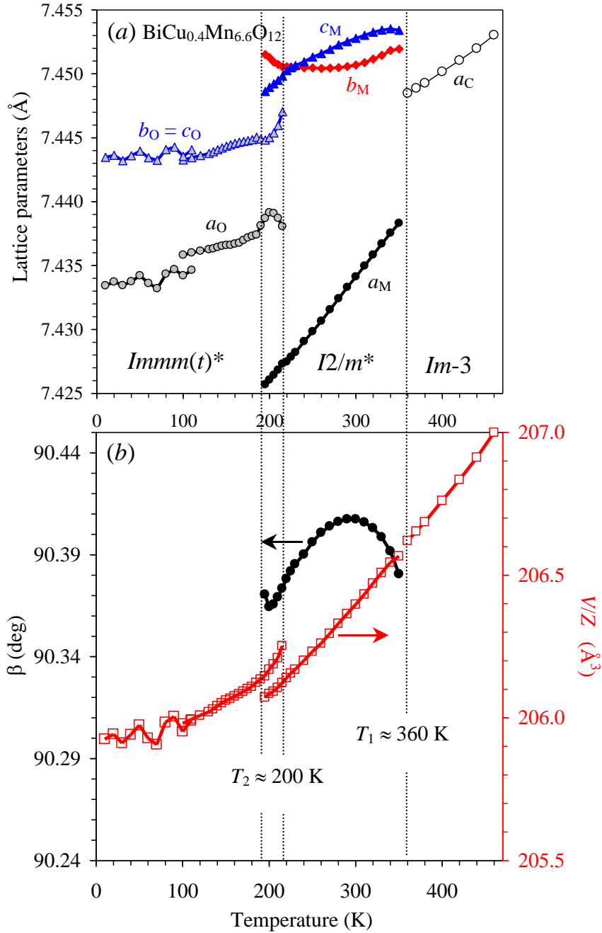
Figure 7. Temperature dependence of (a) the lattice parameters and (b) monoclinic \beta angle (left-hand axis) and the unit-cell volume ( V/Z ) (right-hand axis) in \text{BiCu}_{0.4}\text{Mn}_{6.6}\text{O}_{12} from laboratory XRPD data (from 10 K to 110 K) and synchrotron XRPD data (from 100 K to 460 K). All measurements were performed on heating. M: monoclinic, C: cubic, O: orthorhombic. Stars indicate the presence of additional incommensurately modulated reflections. \alpha_V = 1.8(2) \times 10^{-5} at 360–440 K in the C phase, \alpha_V = 1.5(3) \times 10^{-5} at 195–330 K in the M phase and \alpha_V = 8.1(1.6) \times 10^{-6} at 100–175 K in the O phase (based on synchrotron XRPD data).
