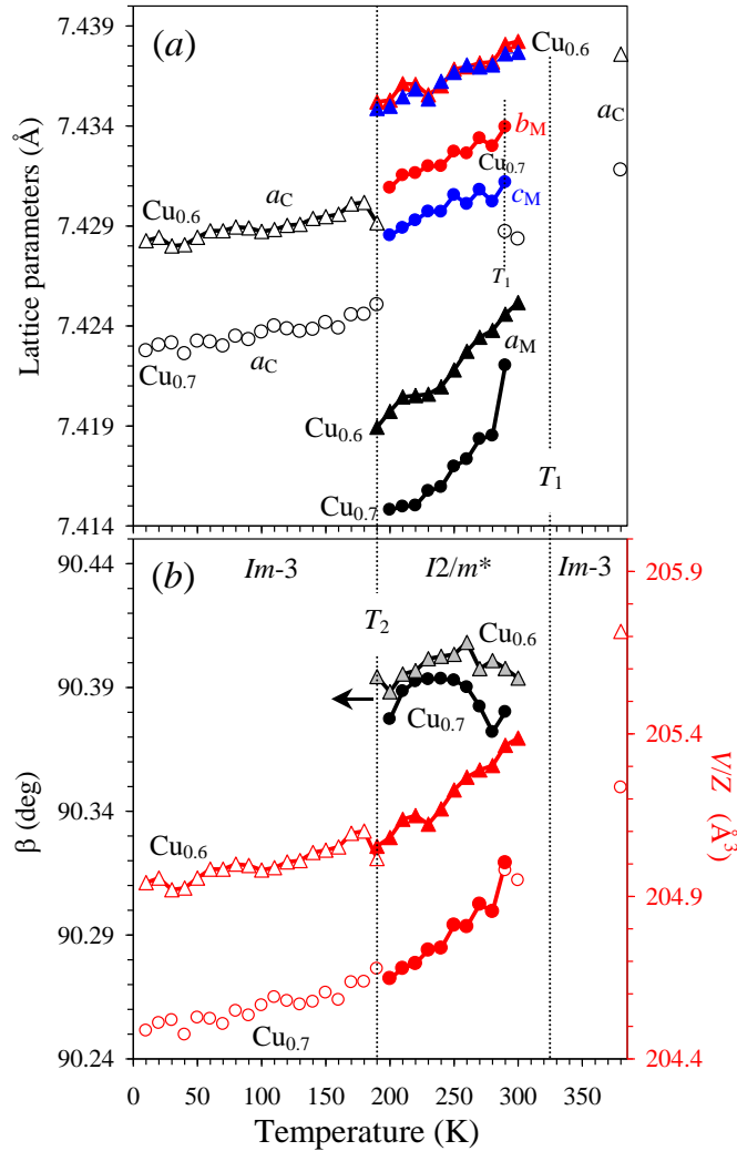
Figure 13. Temperature dependence of (a) the lattice parameters and (b) monoclinic \beta angle (left-hand axis) and the unit-cell volume ( V/Z ) (right-hand axis) in \text{BiCu}_{0.6}\text{Mn}_{6.4}\text{O}_{12} (triangles) and \text{BiCu}_{0.7}\text{Mn}_{6.3}\text{O}_{12} (circles) from laboratory XRPD data (below 300 K). Synchrotron XRPD data were used above 300 K. C: cubic, M: monoclinic. Stars indicate the presence of additional modulated reflections. \alpha_V \sim 4 \times 10^{-6} at 10-180 K in the C phase for x = 0.6 and 0.7.
