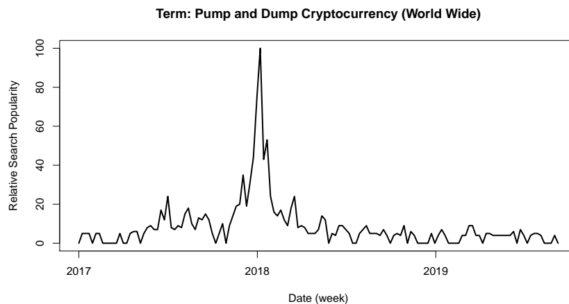
Figure 1: Google Trends results from searching for pump and dump cryptocurrency.
