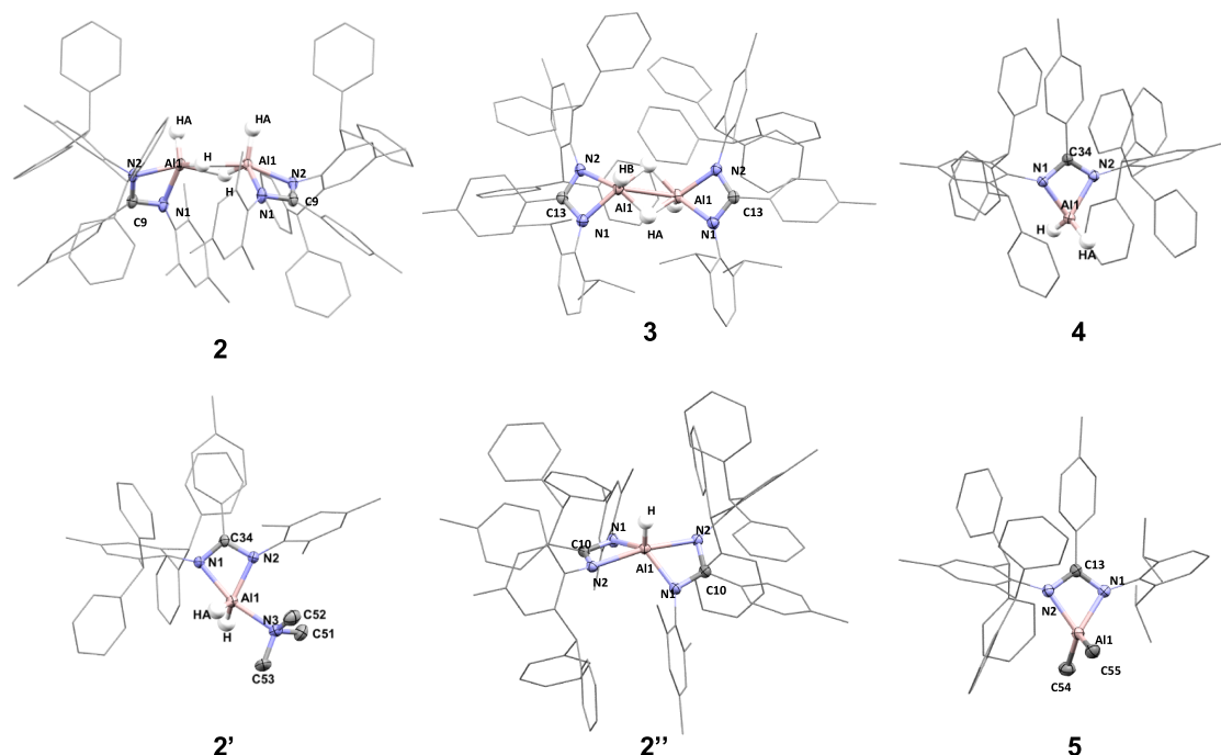
Figure 4. Solid-state structures of compounds 2, 2', 2'', and 3–5. See the SI for a table of key bond lengths and bond angles (Table S1).
