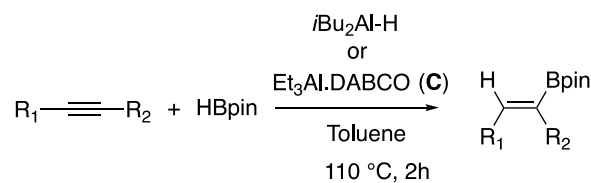
Figure 1. Examples of catalysts or precatalysts for hydroboration reactions.
