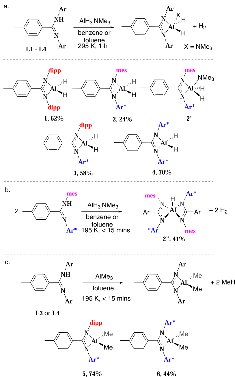
Figure 3. Synthesis of (a) aluminum dihydrides 1–4 and 2'. (b) Aluminum monohydride 2''. (c) Aluminum dimethyl compounds 5 and 6.
